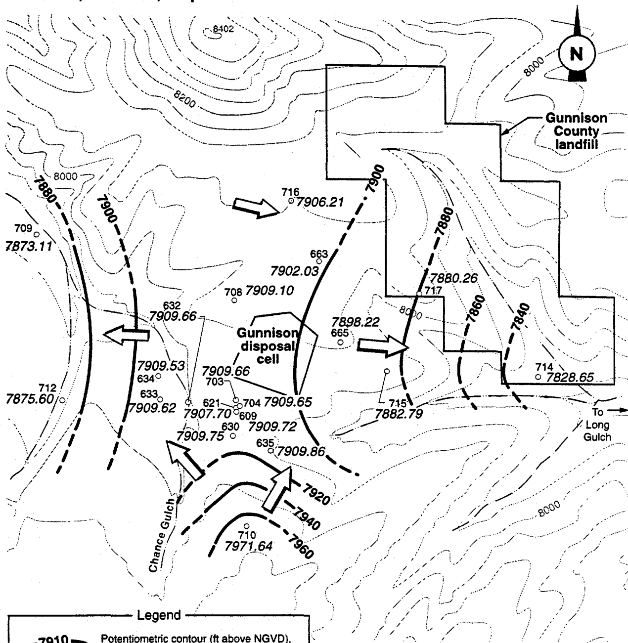
Figure 2.5 Potentiometric Map of the Lower Tertiary Gravel Aquifer Gunnison, Colorado, Disposal Site
