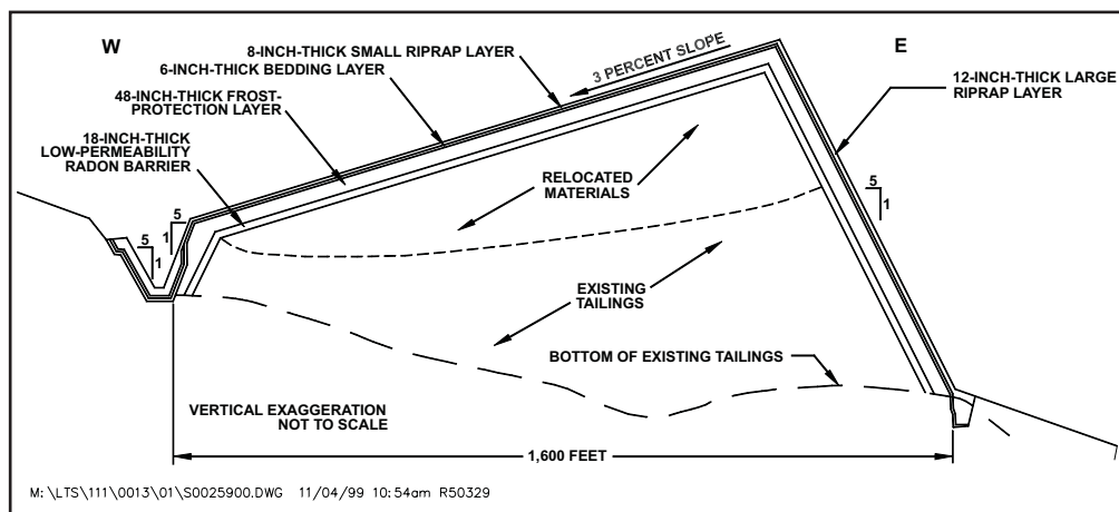
West-East Cross Section of Maybell Disposal Cell
