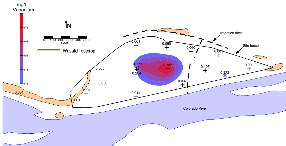
Figure 12. Vanadium Distribution in Alluvial Aquifer—Old Rifle, May 1998
