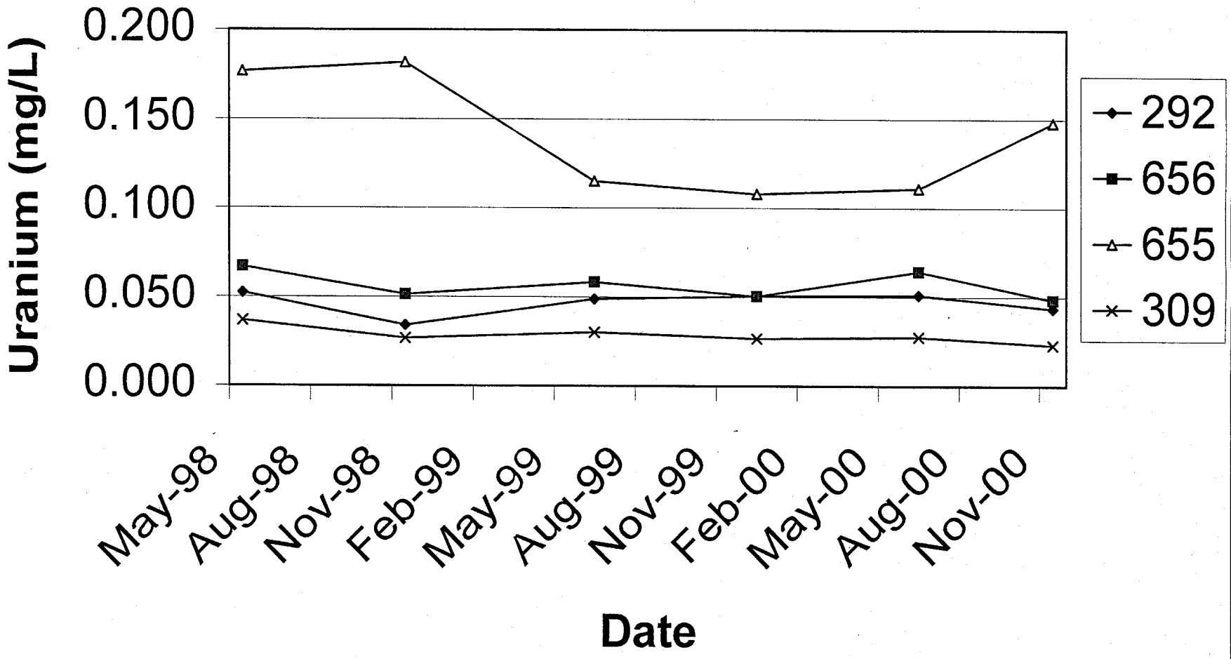
Figure 8. Time-Concentration Plot for Uranium for Old Rifle Wells 292, 309, 655, and 656
