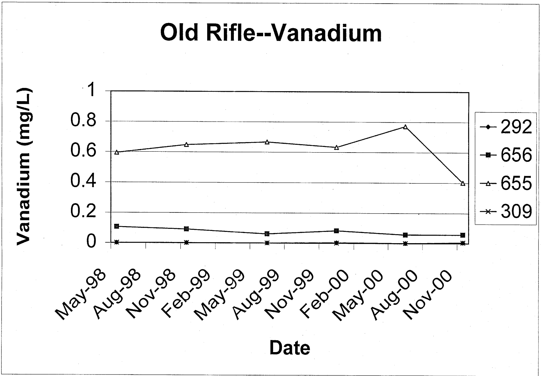
Figure 9. Time-Concentration Plot for Vanadium for Old Rifle Wells 292, 309, 655, and 656
