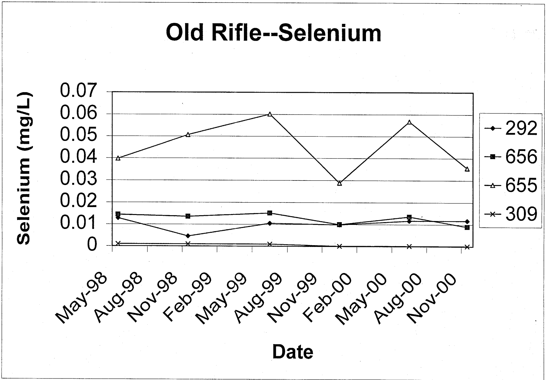
Figure 5. Time-Concentration Plot for Selenium for Old Rifle Wells 292, 309, 655, and 656
