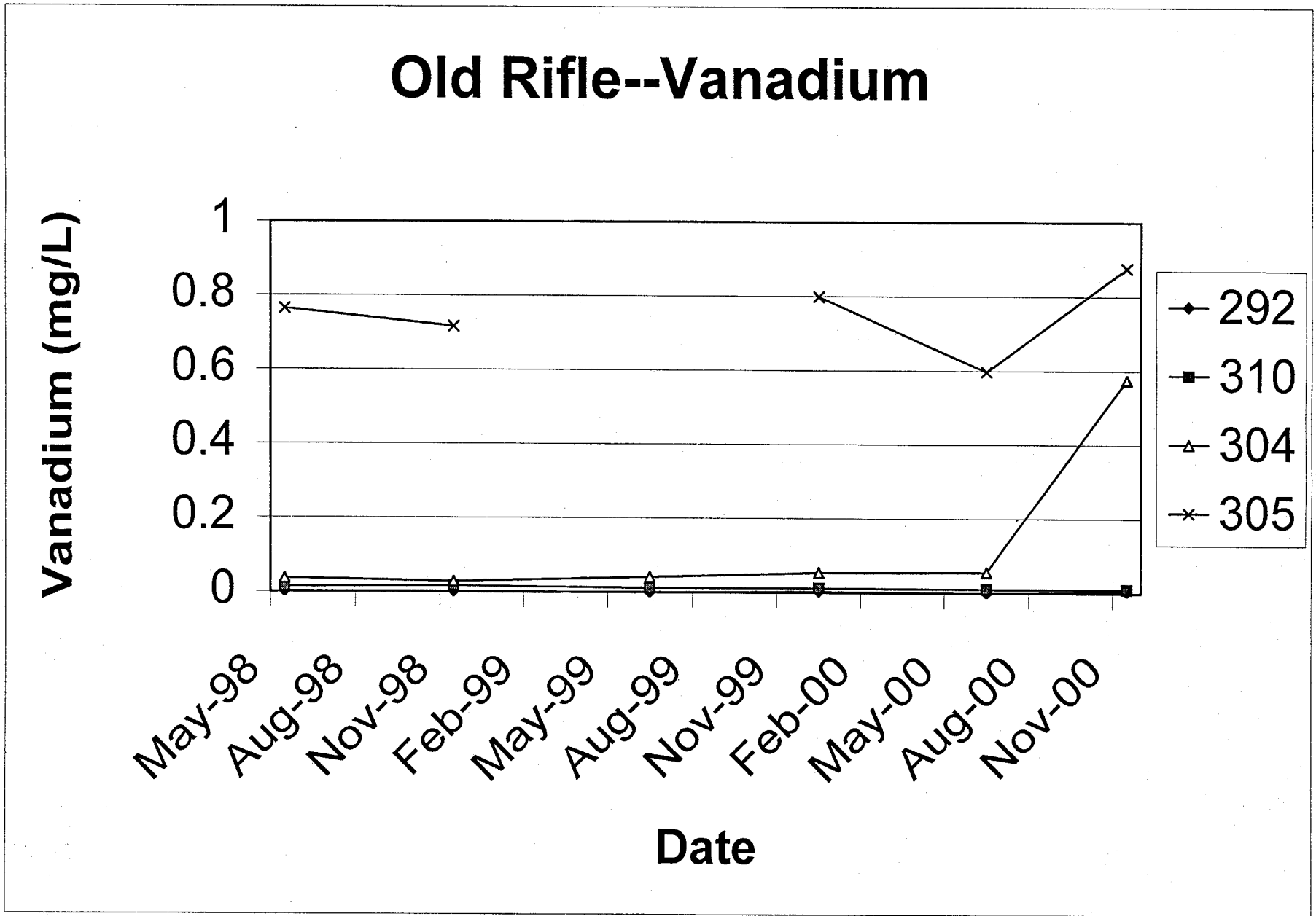
Figure 8. Time-Concentration Plot for Vanadium for Old Rifle Wells 292, 304, 305, and 310
