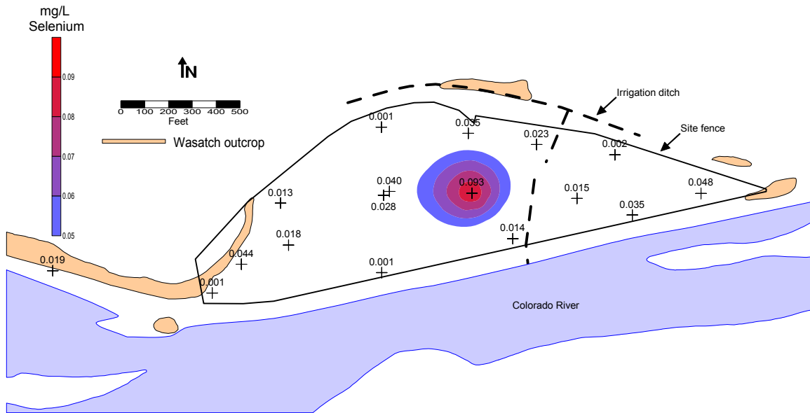
Figure 11. Selenium Distribution in Alluvial Aquifer—Old Rifle, May 1998
