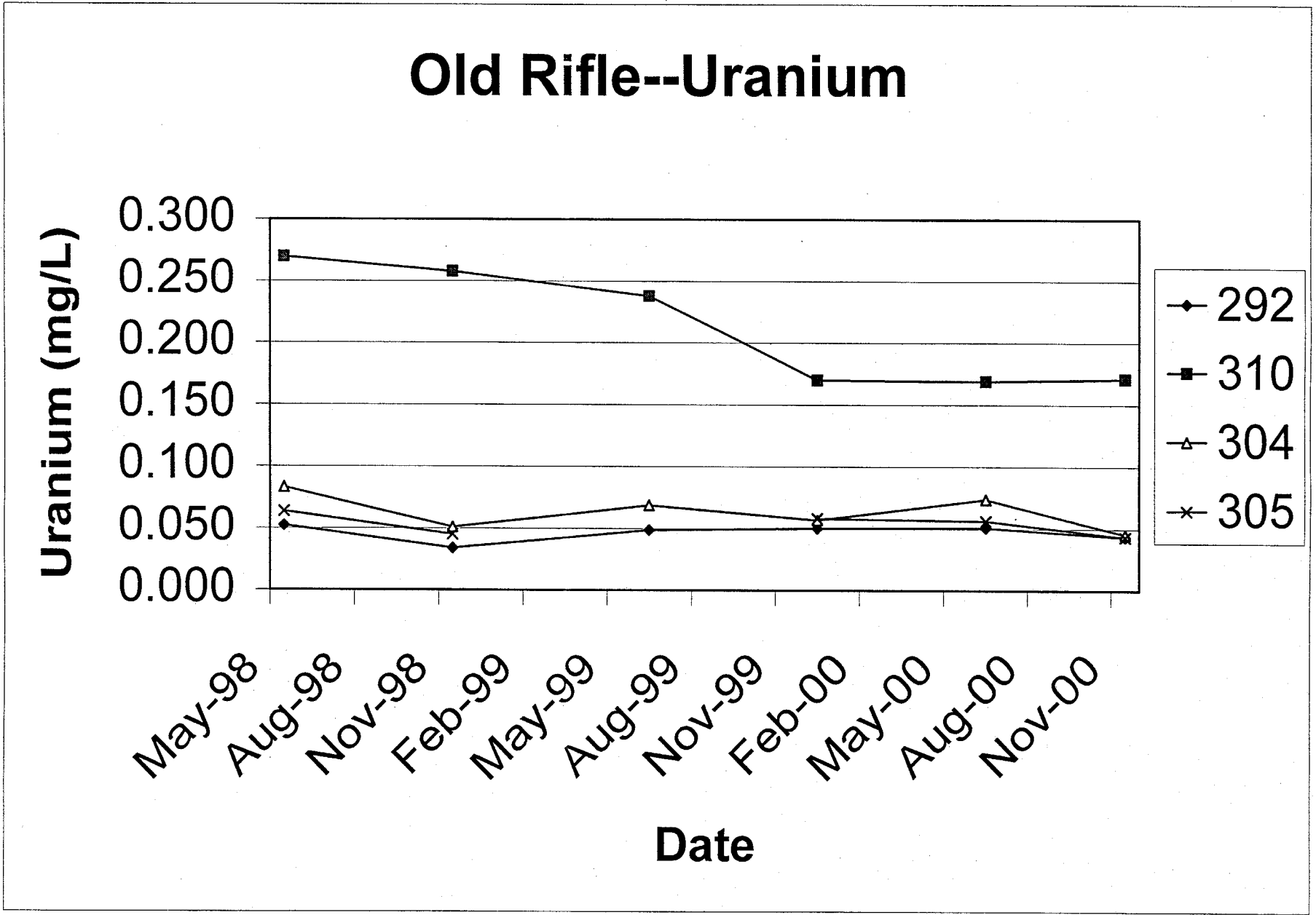
Figure 7. Time-Concentration Plot for Uranium for Old Rifle Wells 292, 304, 305, and 310
