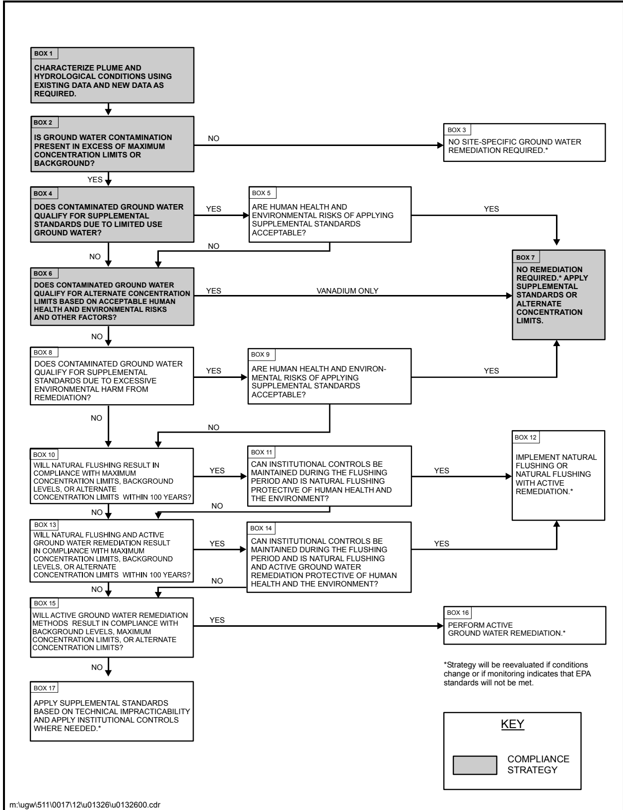
Figure 2. Compliance Selection Framework for Vanadium at the Old Rifle Site
