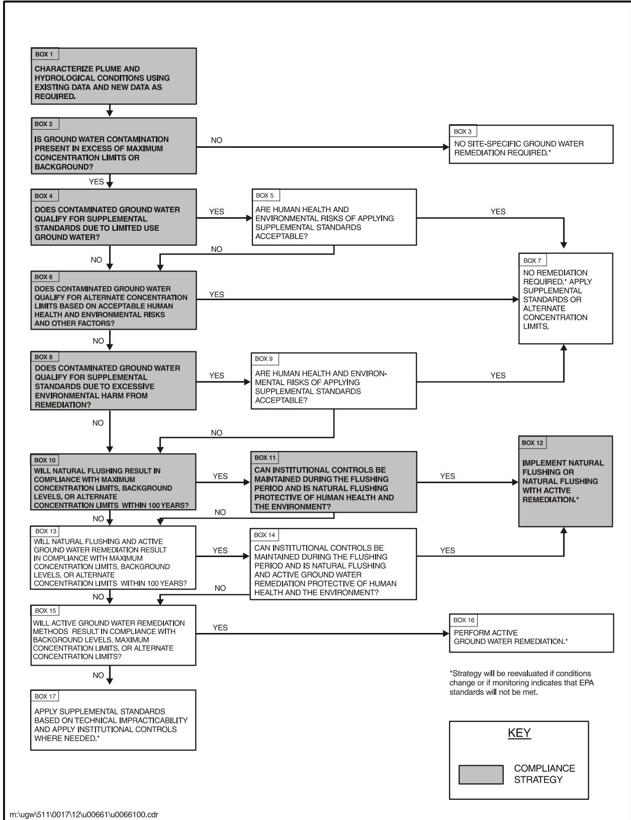
Figure 1. Compliance Selection Framework for Selenium and Uranium at the Old Rifle Site
