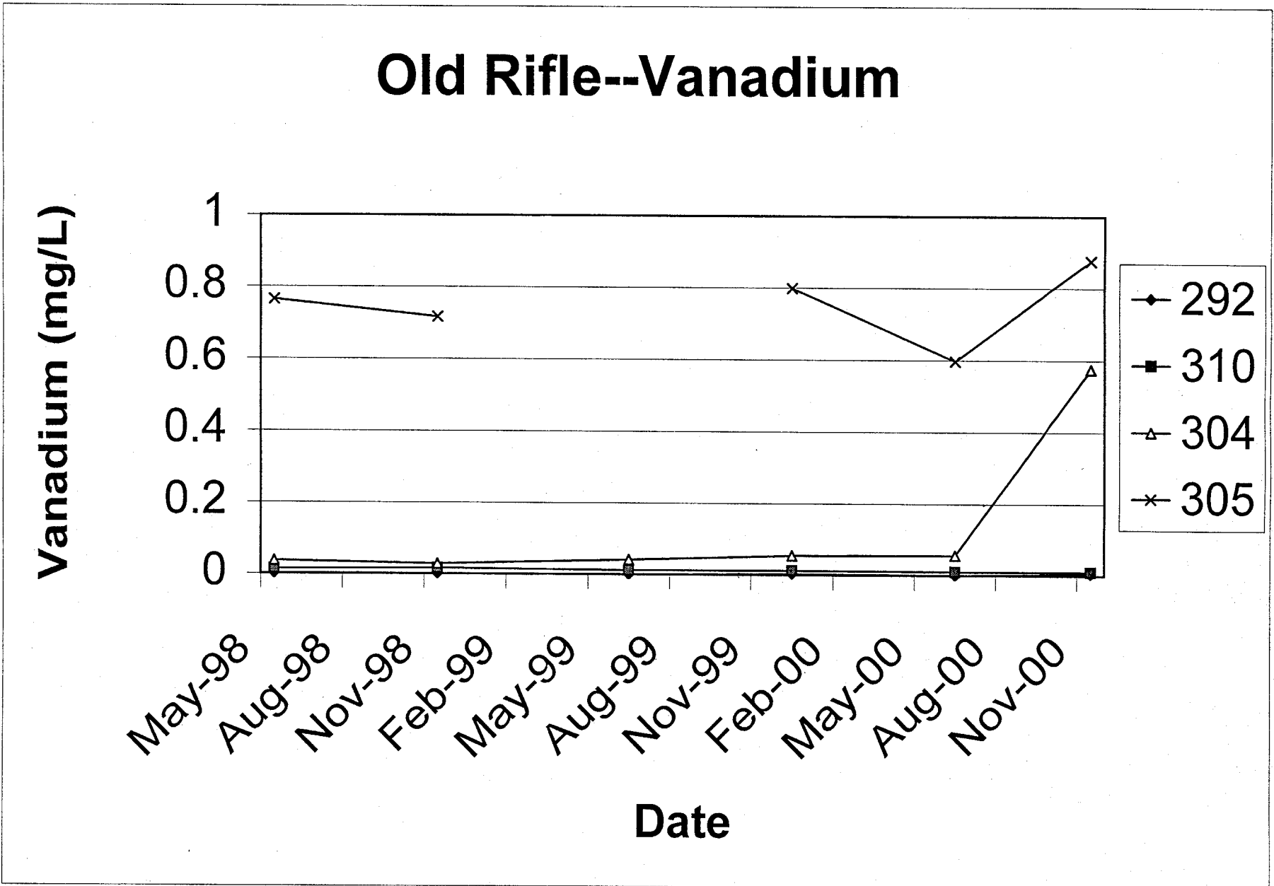
Figure 9. Time-Concentration Plot for Vanadium for Old Rifle Wells 292, 304, 305, and 310
