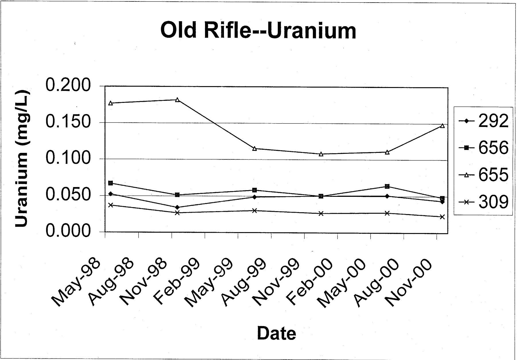
Figure 7. Time-Concentration Plot for Uranium for Old Rifle Wells 292, 309, 655, and 656
