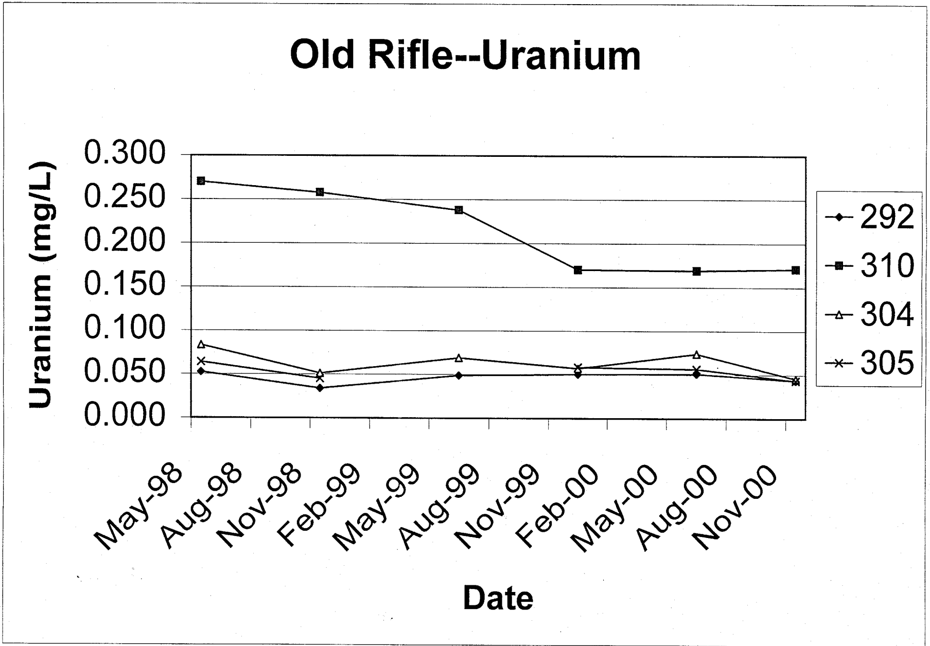
Figure 6. Time-Concentration Plot for Uranium for Old Rifle Wells 292, 304, 305, and 310
