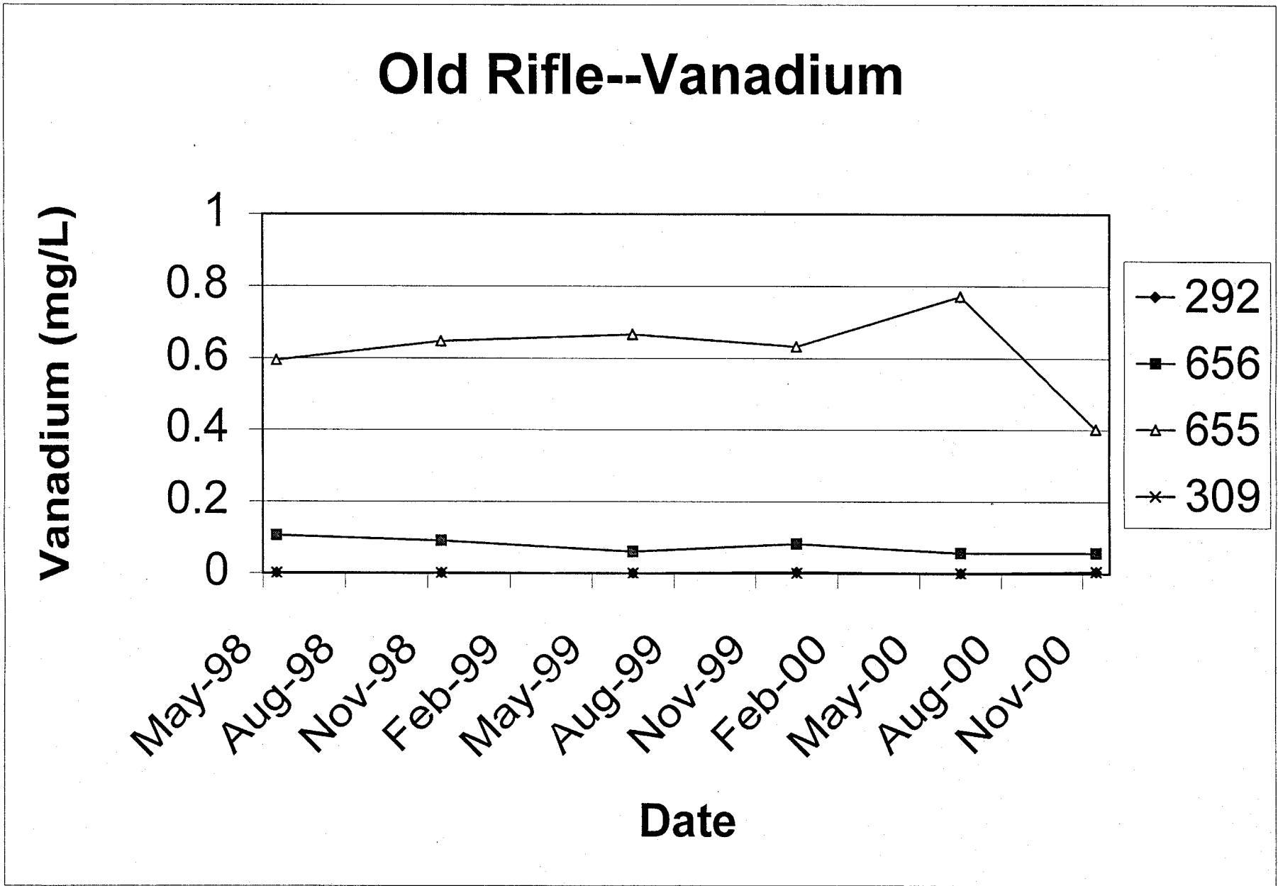
Figure 10. Time-Concentration Plot for Vanadium for Old Rifle Wells 292, 309, 655, and 656
