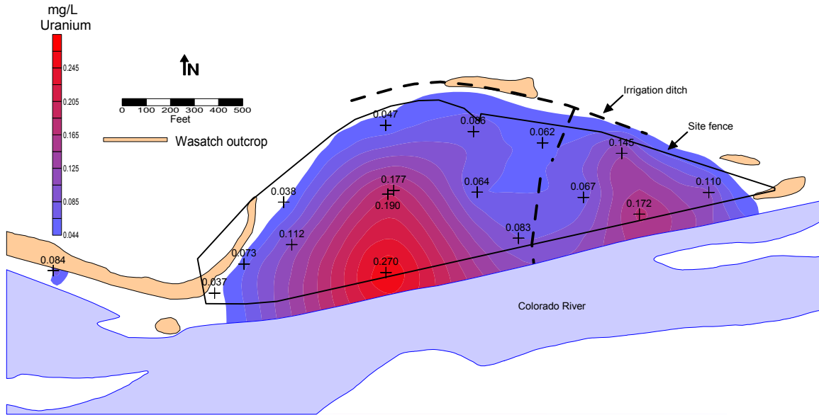
Figure 10. Uranium Distribution in Alluvial Aquifer—Old Rifle, May 1998
