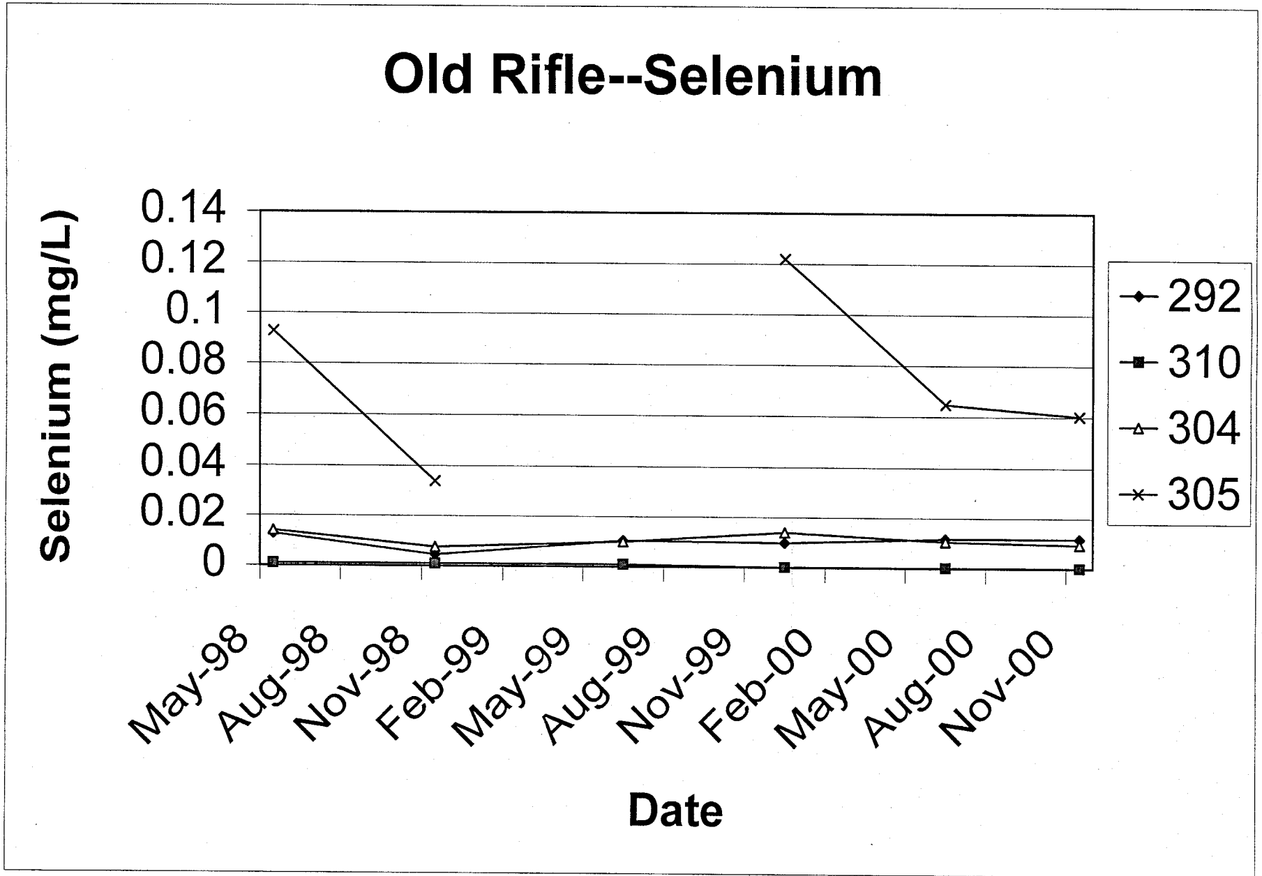
Figure 5. Time-Concentration Plot for Selenium for Old Rifle Wells 292, 304, 305, and 310
