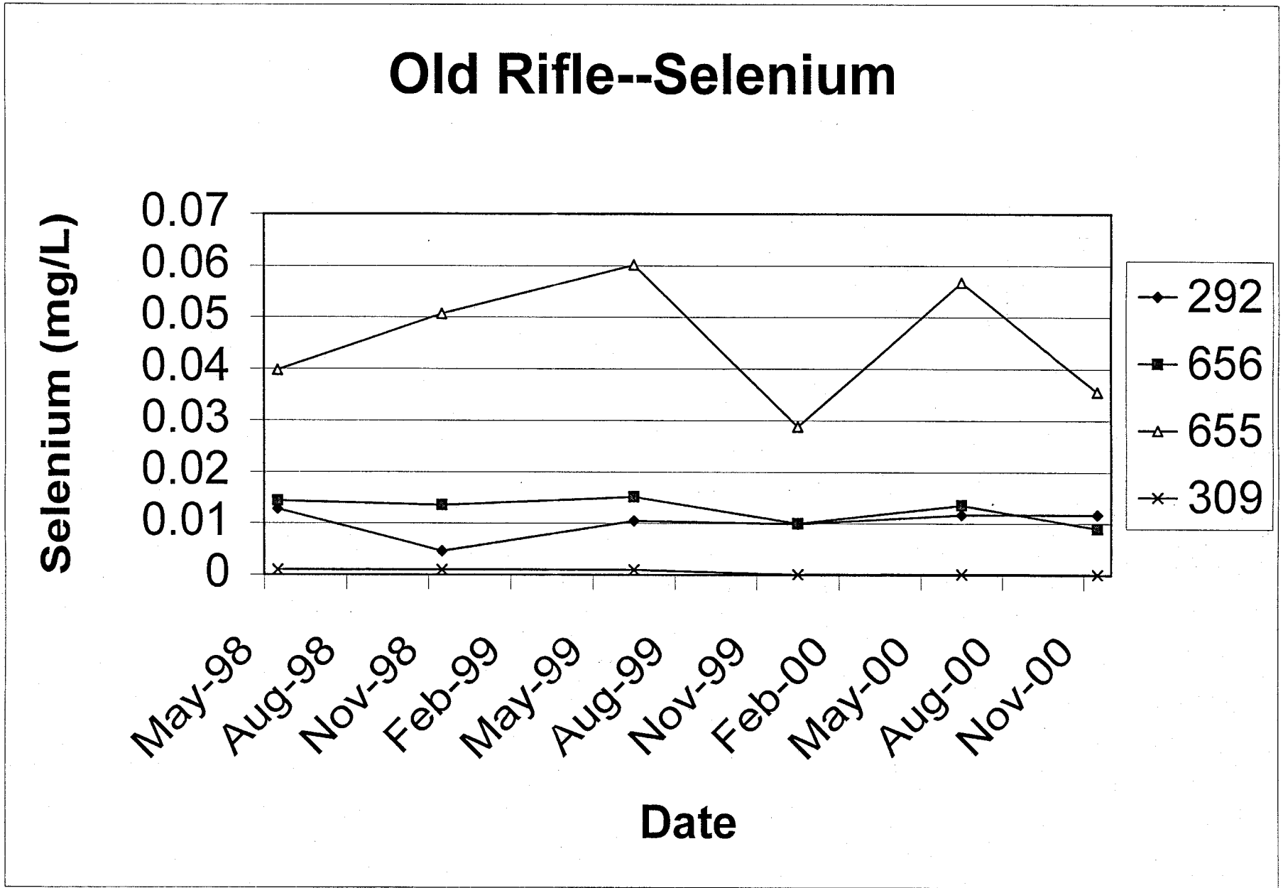
Figure 6. Time-Concentration Plot for Selenium for Old Rifle Wells 292, 309, 655, and 656
