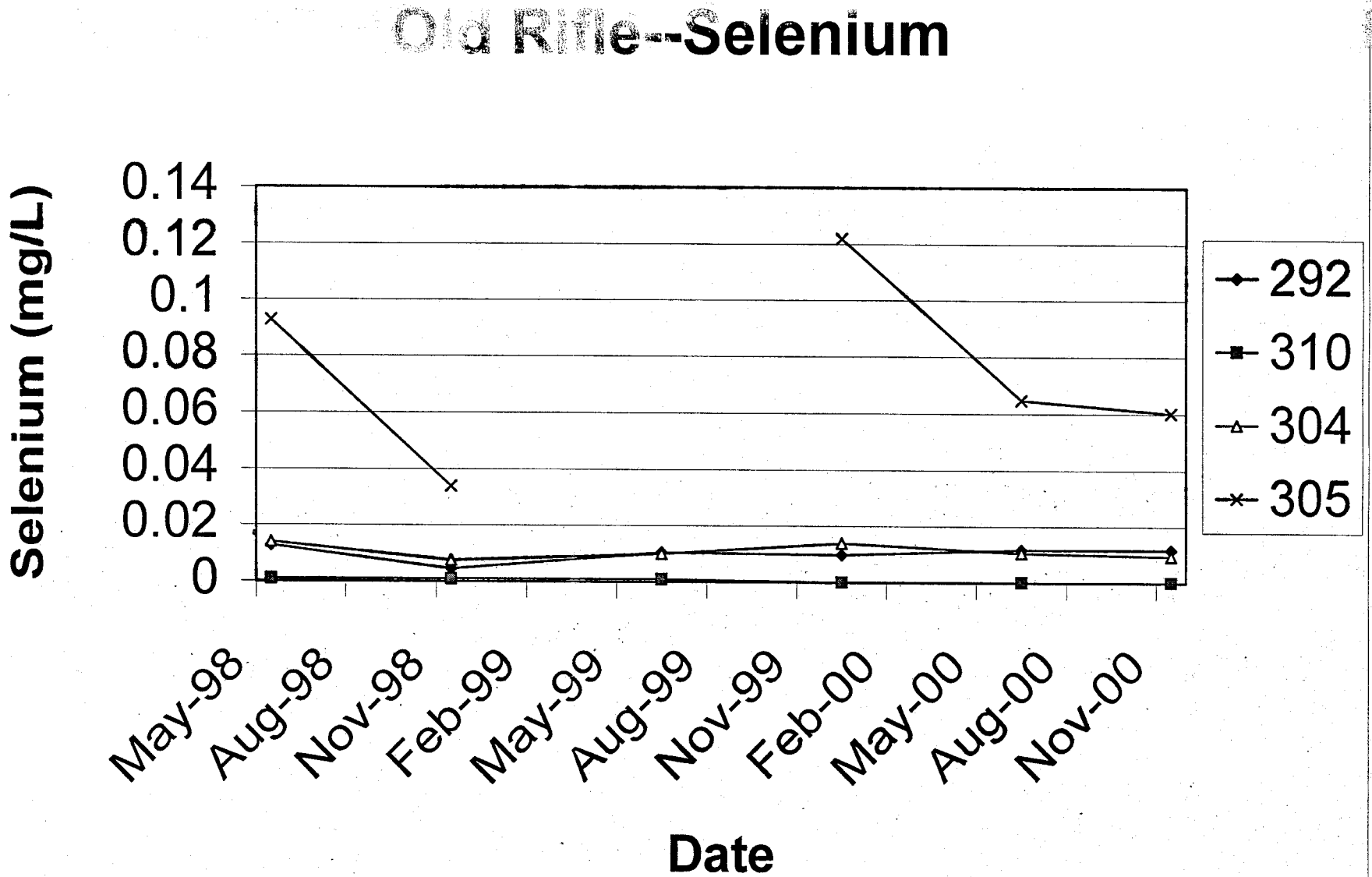
Figure 4. Time-Concentration Plot for Selenium for Old Rifle Wells 292, 304, 305, and 310
