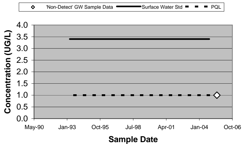
88104 - Chloroform (Unfiltered)
