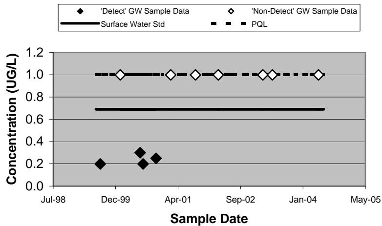
90299 - Tetrachloroethene (Unfiltered)
