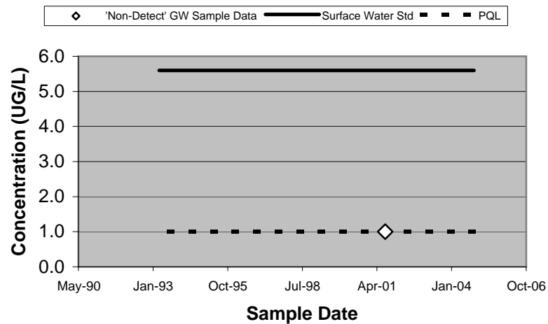
37401 - Chloromethane (Unfiltered)
