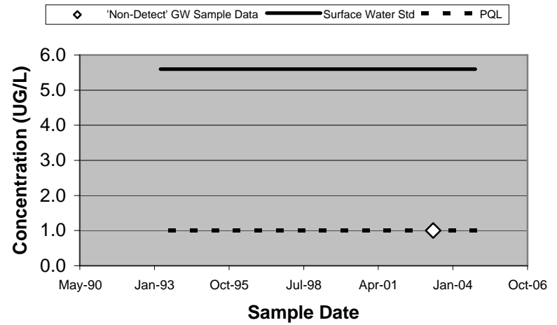
70299 - Chloromethane (Unfiltered)
