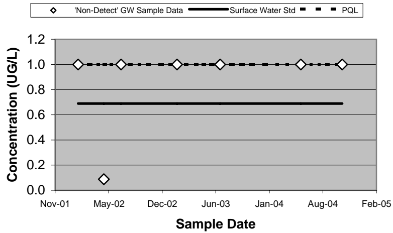
99401 - Tetrachloroethene (Unfiltered)
