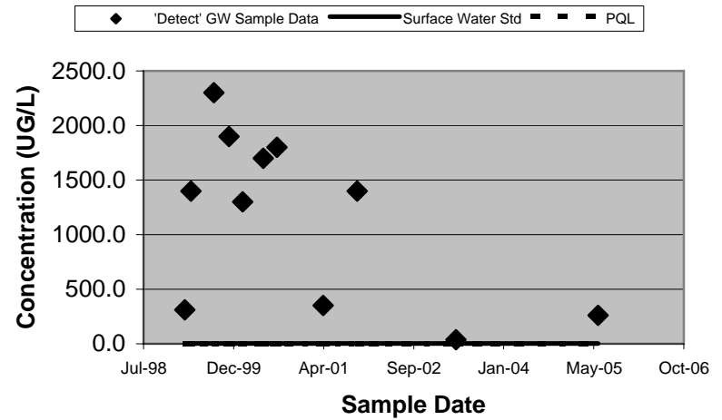
15699 - Trichloroethene (Unfiltered)
