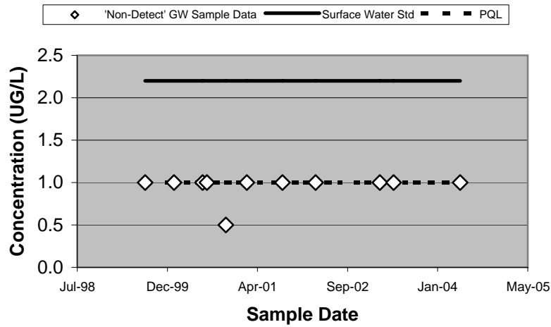
90299 - Benzene (Unfiltered)
