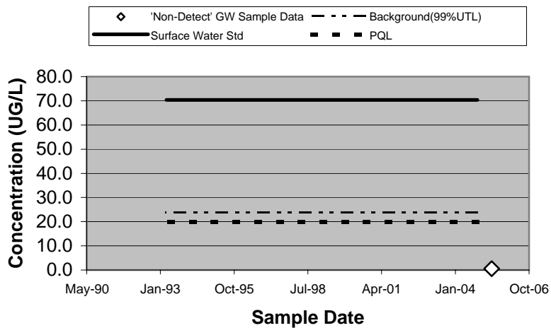
20205 - Nickel (Filtered)
