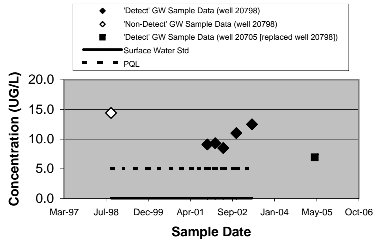
20798/20705 - Arsenic (Filtered)
