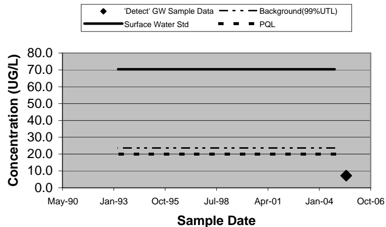
15699 - Nickel (Filtered)
