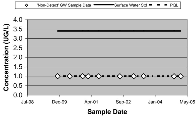
40399 - Chloroform (Unfiltered)
