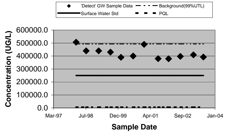
00797 - Sulfate (Unfiltered)
