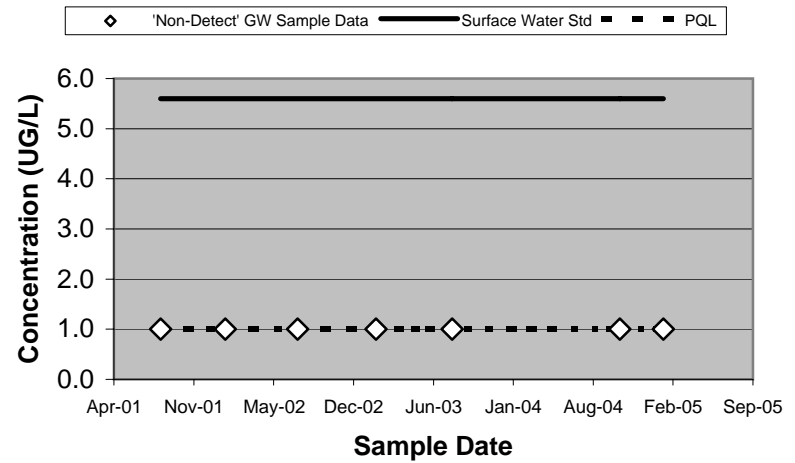
37501 - Chloromethane (Unfiltered)
