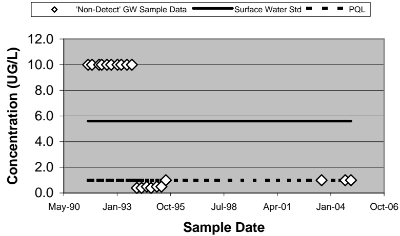
2187 - Chloromethane (Unfiltered)
