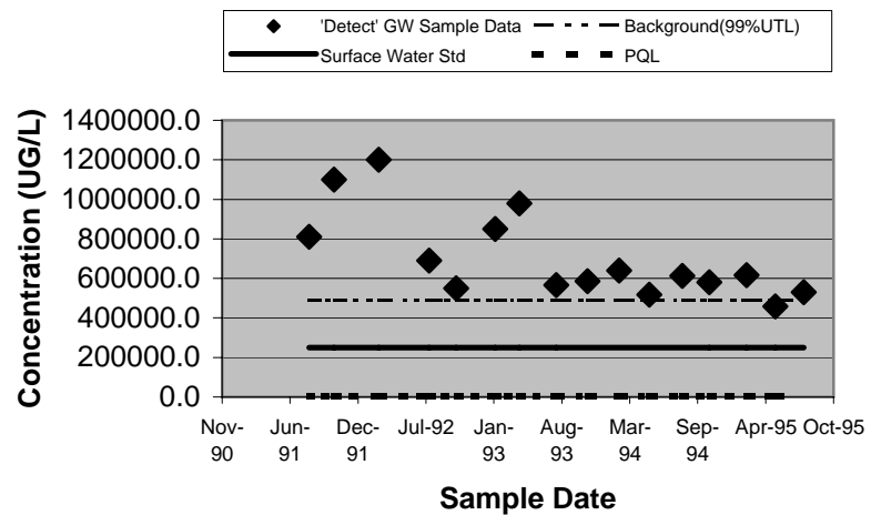
2187 - Sulfate (Unfiltered)
