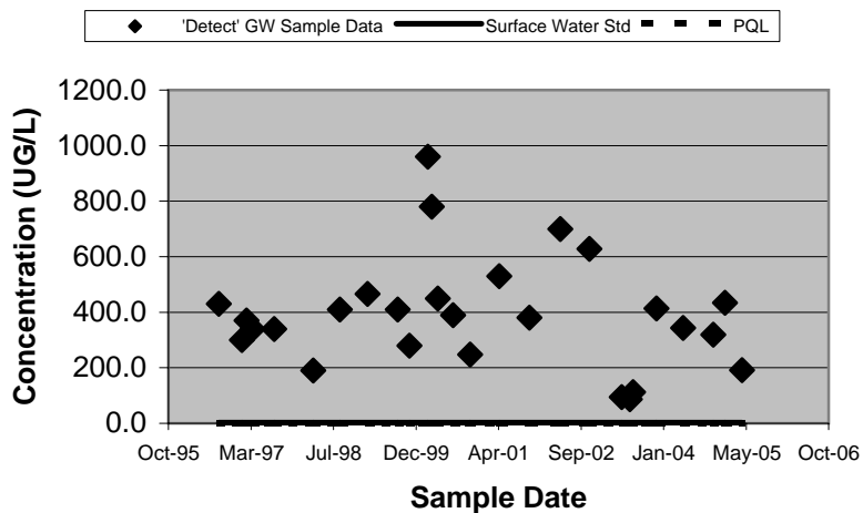
23296 - Trichloroethene (Unfiltered)
