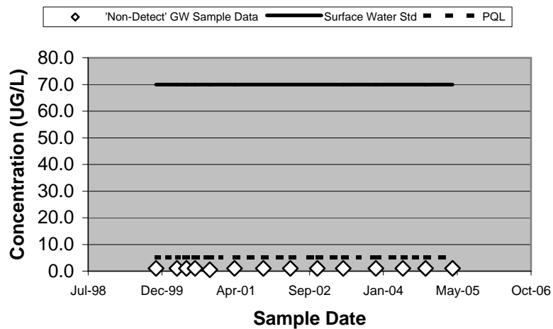
95099 - cis-1,2-Dichloroethene (Unfiltered)
