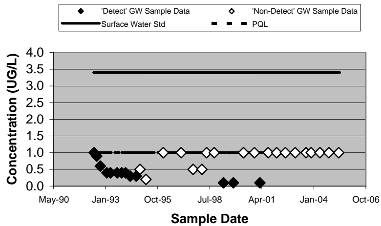
04091 - Chloroform (Unfiltered)
