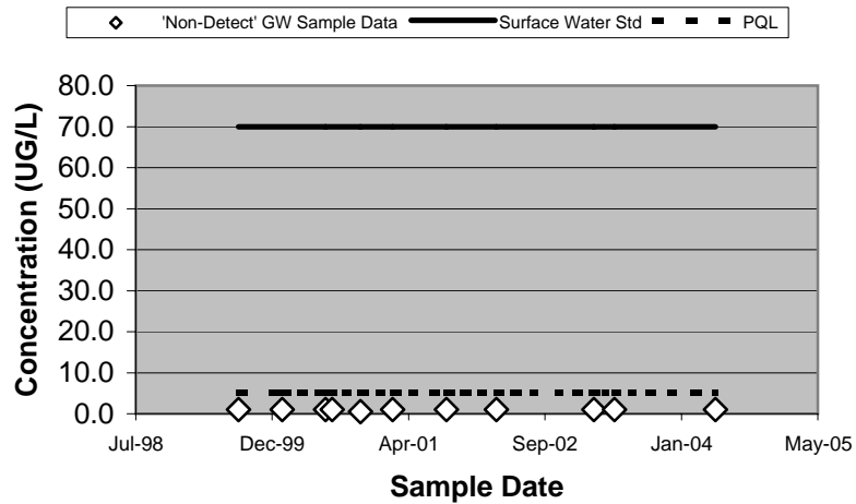
90299 - cis-1,2-Dichloroethene (Unfiltered)
