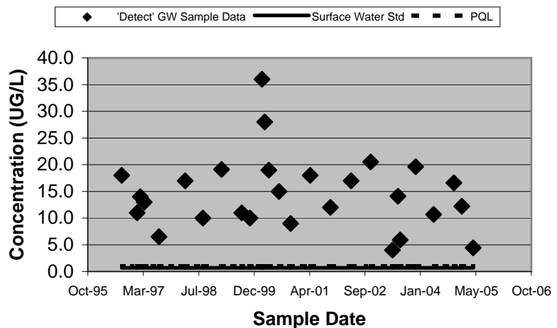
23296 - Tetrachloroethene (Unfiltered)
