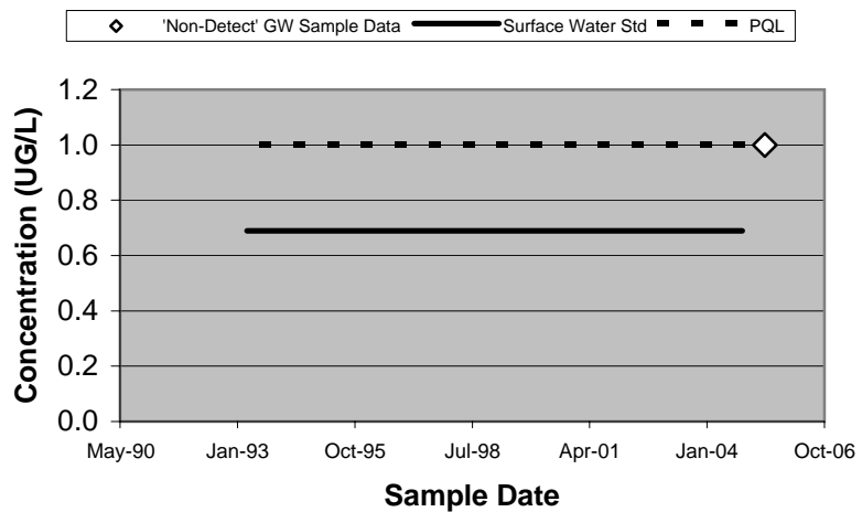
20205 - Tetrachloroethene (Unfiltered)
