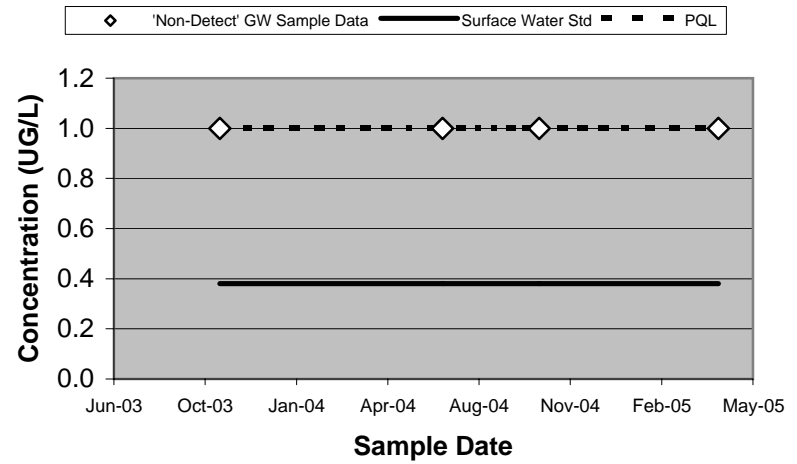
33703 - 1,2-Dichloroethane (Unfiltered)
