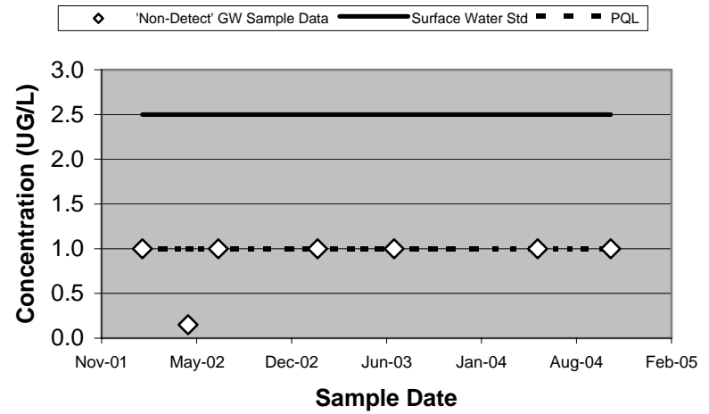
99401 - Trichloroethene (Unfiltered)
