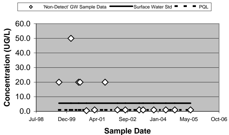
90399 - Chloromethane (Unfiltered)
