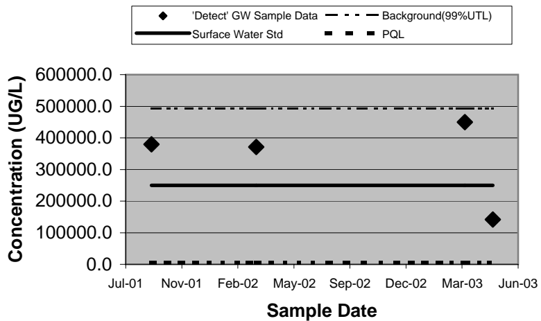
90299 - Sulfate (Unfiltered)
