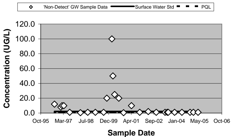
23296 - Benzene (Unfiltered)
