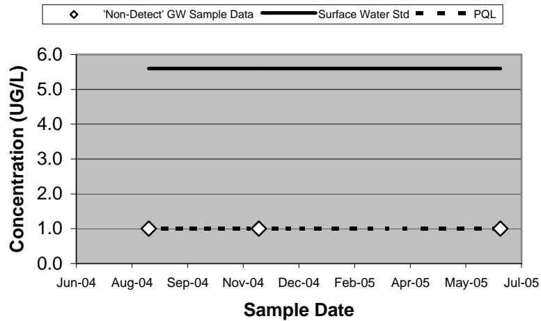
10304 - Chloromethane (Unfiltered)
