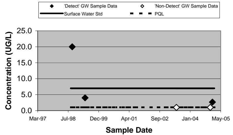
20598 - 1,1-Dichloroethene (Unfiltered)
