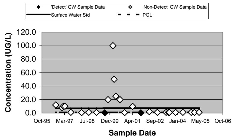
23296 - 1,1-Dichloroethene (Unfiltered)
