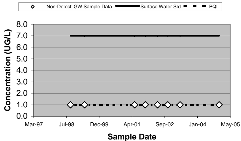
20298 - 1,1-Dichloroethene (Unfiltered)
