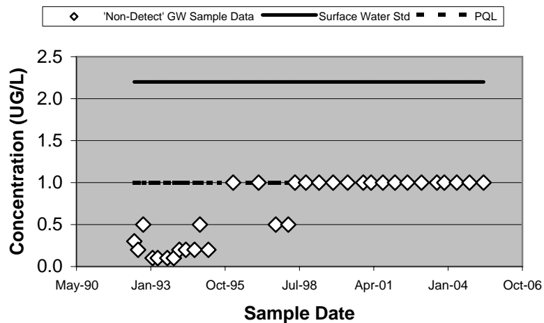
04091 - Benzene (Unfiltered)
