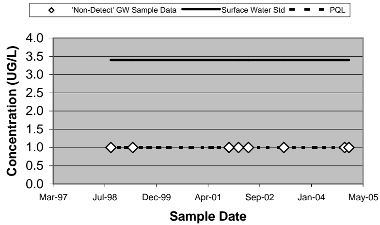
20798 - Chloroform (Unfiltered)
