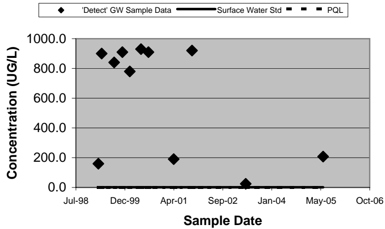
15699 - Tetrachloroethene (Unfiltered)
