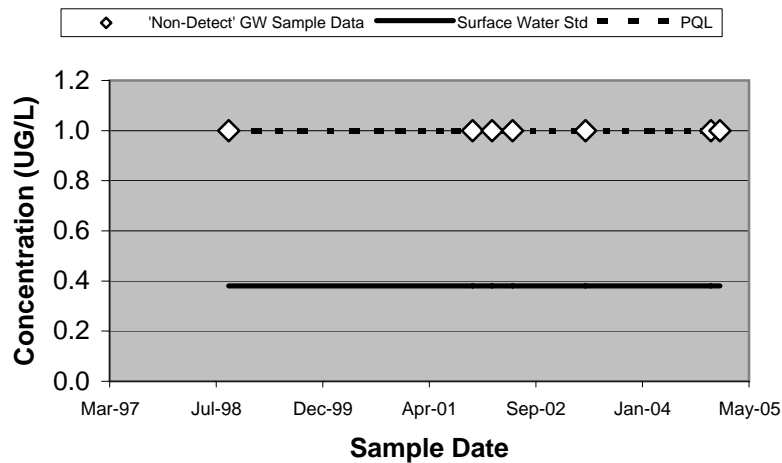
20798 - 1,2-Dichloroethane (Unfiltered)
