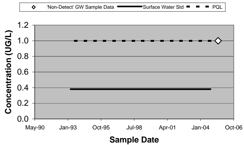
91305 - 1,2-Dichloroethane (Unfiltered)
