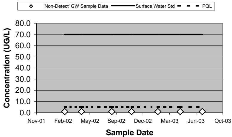
88101 - cis-1,2-Dichloroethene (Unfiltered)
