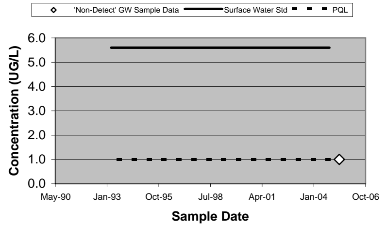
20205 - Chloromethane (Unfiltered)
