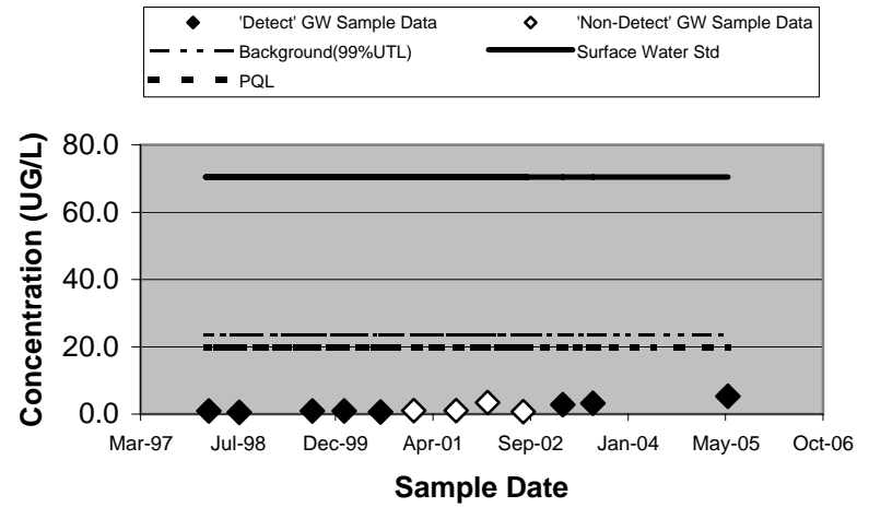
00797 - Nickel (Filtered)
