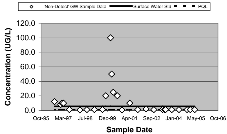
23296 - Chloromethane (Unfiltered)
