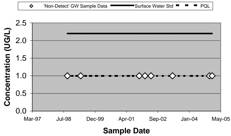
20798 - Benzene (Unfiltered)
