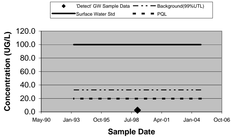
00797 - Nickel (Unfiltered)
