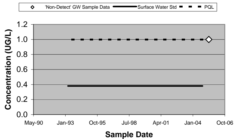
20505 - 1,2-Dichloroethane (Unfiltered)
