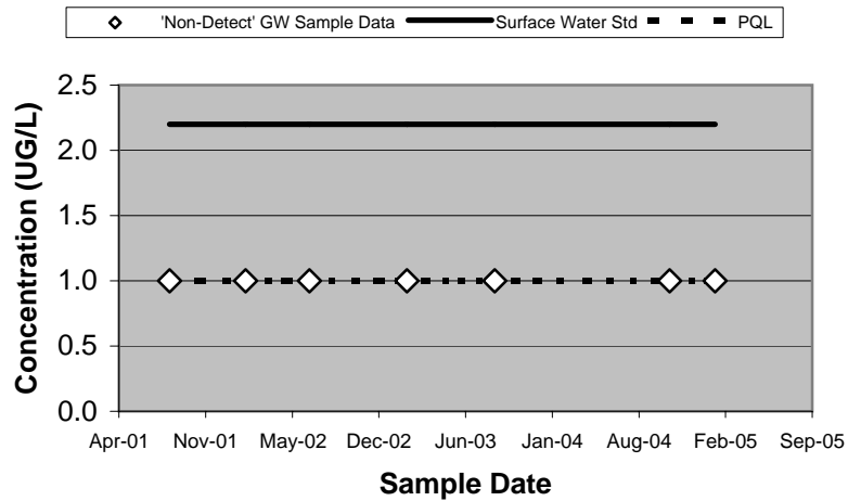
37701 - Benzene (Unfiltered)
