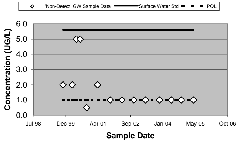
95199 - Chloromethane (Unfiltered)
