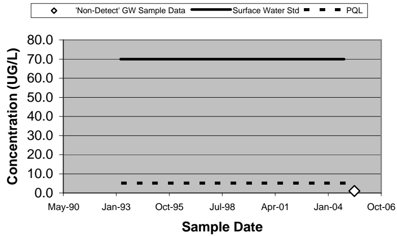
20205 - cis-1,2-Dichloroethene (Unfiltered)
