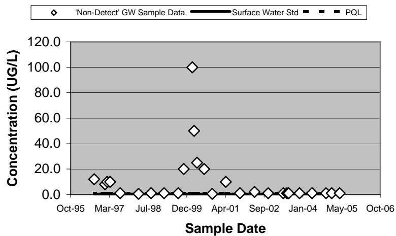
23296 - 1,2-Dichloroethane (Unfiltered)
