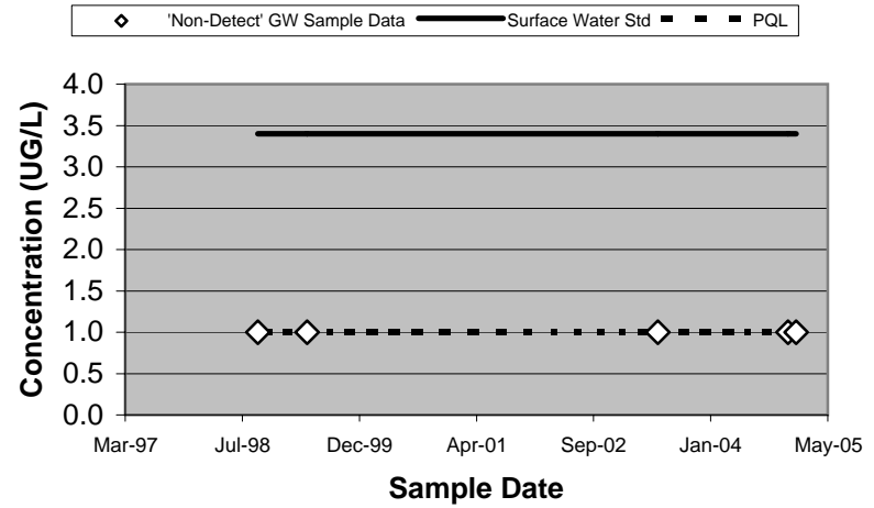
20598 - Chloroform (Unfiltered)
