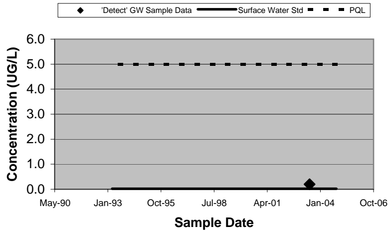
20298 - Arsenic (Filtered)
