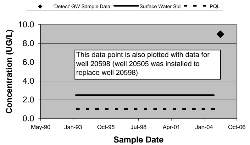
20505 - Trichloroethene (Unfiltered)
