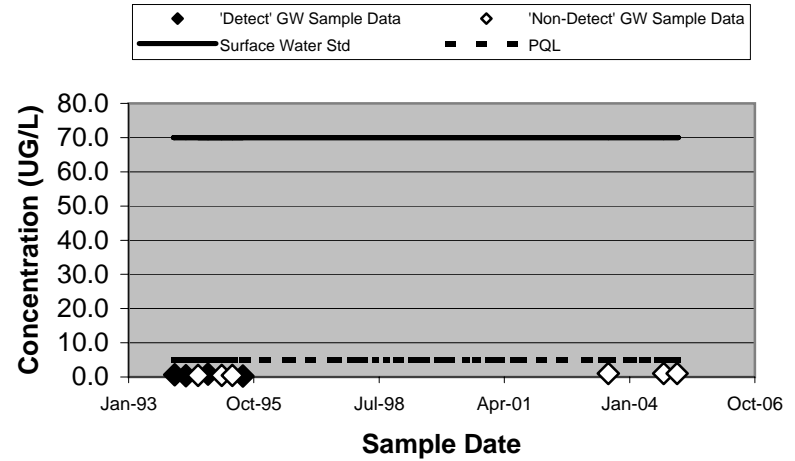
2187 - cis-1,2-Dichloroethene (Unfiltered)
