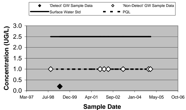
20798 - Trichloroethene (Unfiltered)
