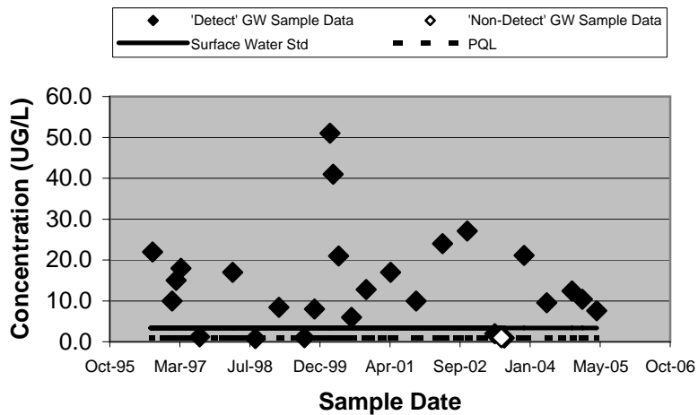
23296 - Chloroform (Unfiltered)
