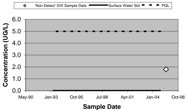
15699 - Arsenic (Filtered)
