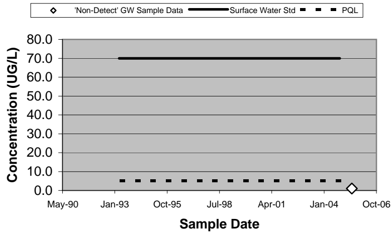
99405 - cis-1,2-Dichloroethene (Unfiltered)
