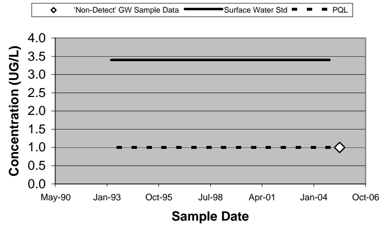
20505 - Chloroform (Unfiltered)
