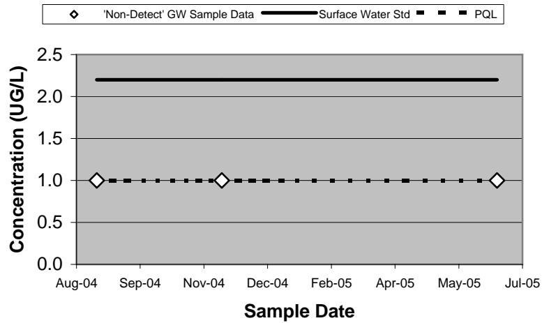
11104 - Benzene (Unfiltered)
