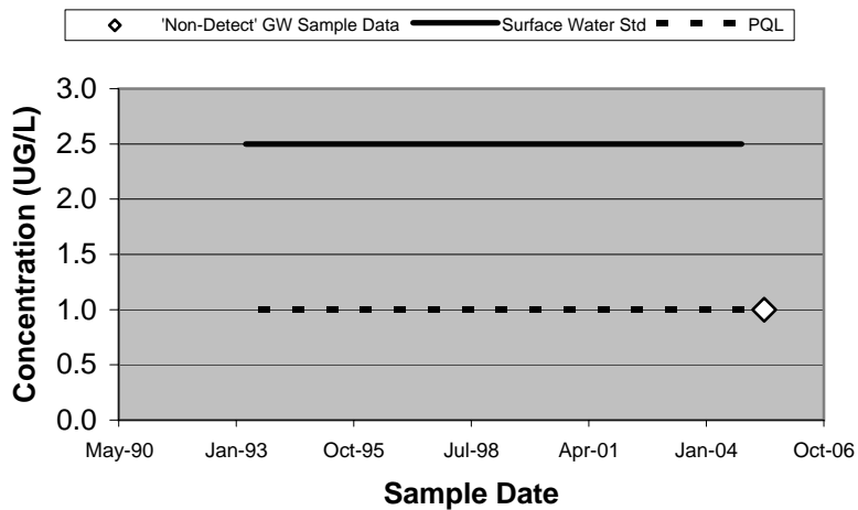
20205 - Trichloroethene (Unfiltered)
