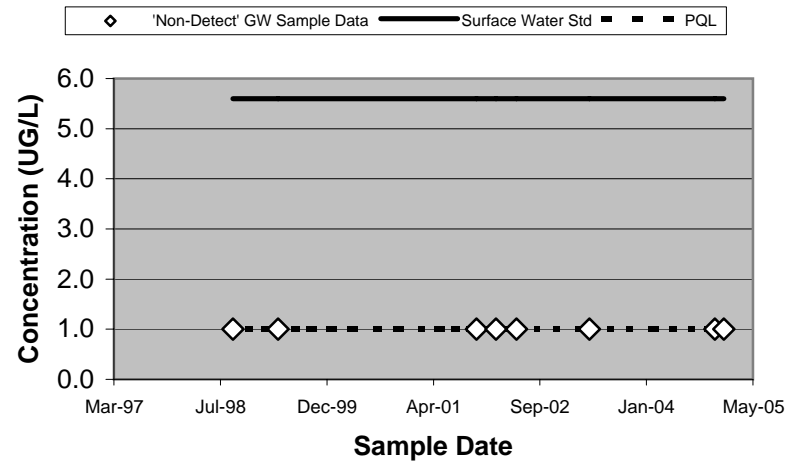
20798 - Chloromethane (Unfiltered)
