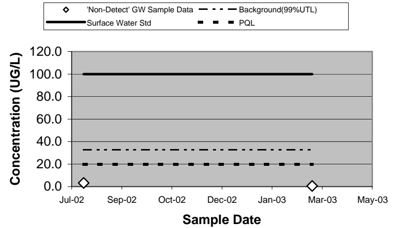
90399 - Nickel (Unfiltered)
