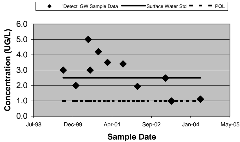
90299 - Trichloroethene (Unfiltered)
