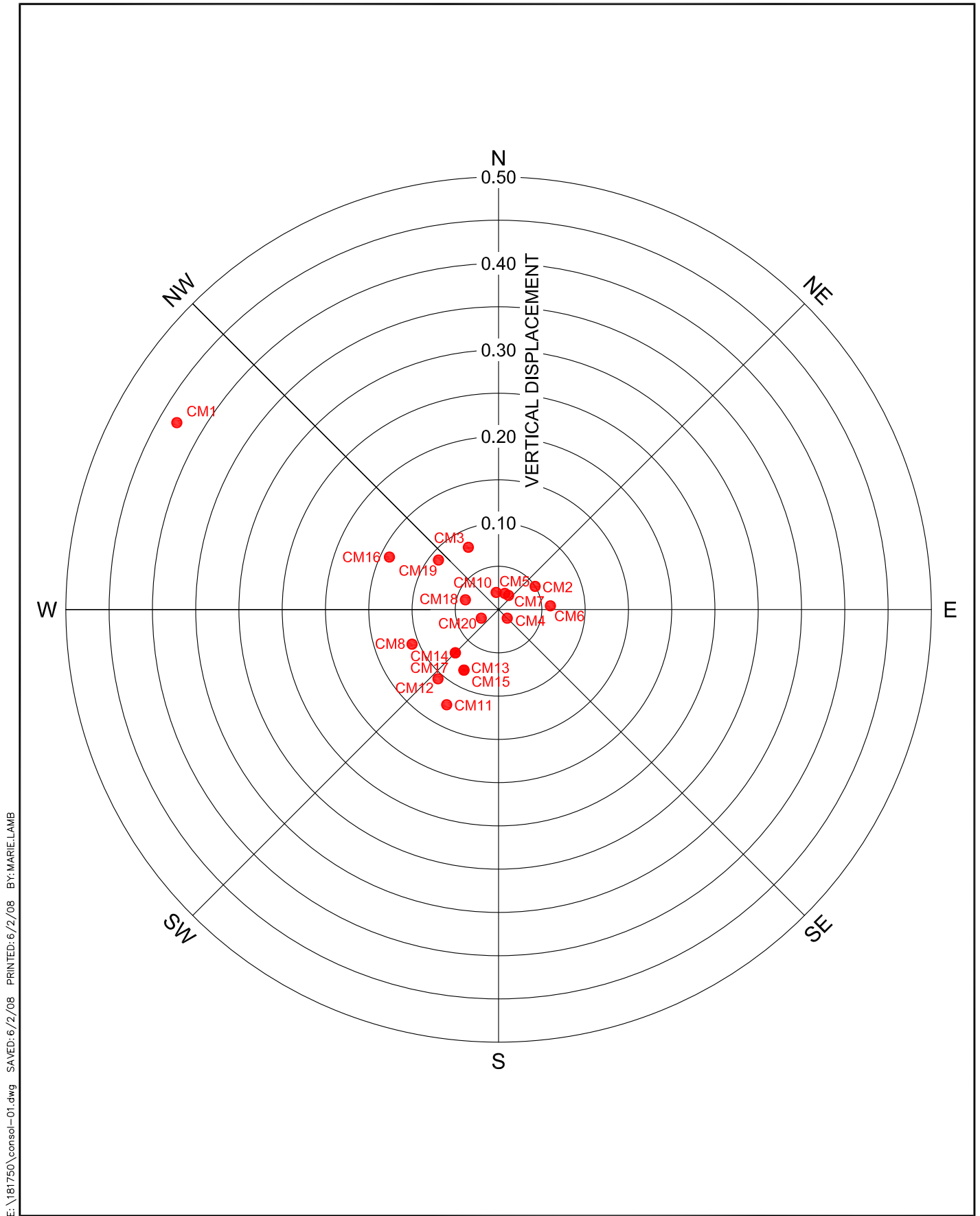
FIGURE F.1 ROCKY FLATS SITE ORIGINAL LANDFILL SETTLEMENT MONITORS MONTHLY SURVEY APRIL 04 2008 COMPARISON TO BASE SURVEY SEPTEMBER 28, 2007
