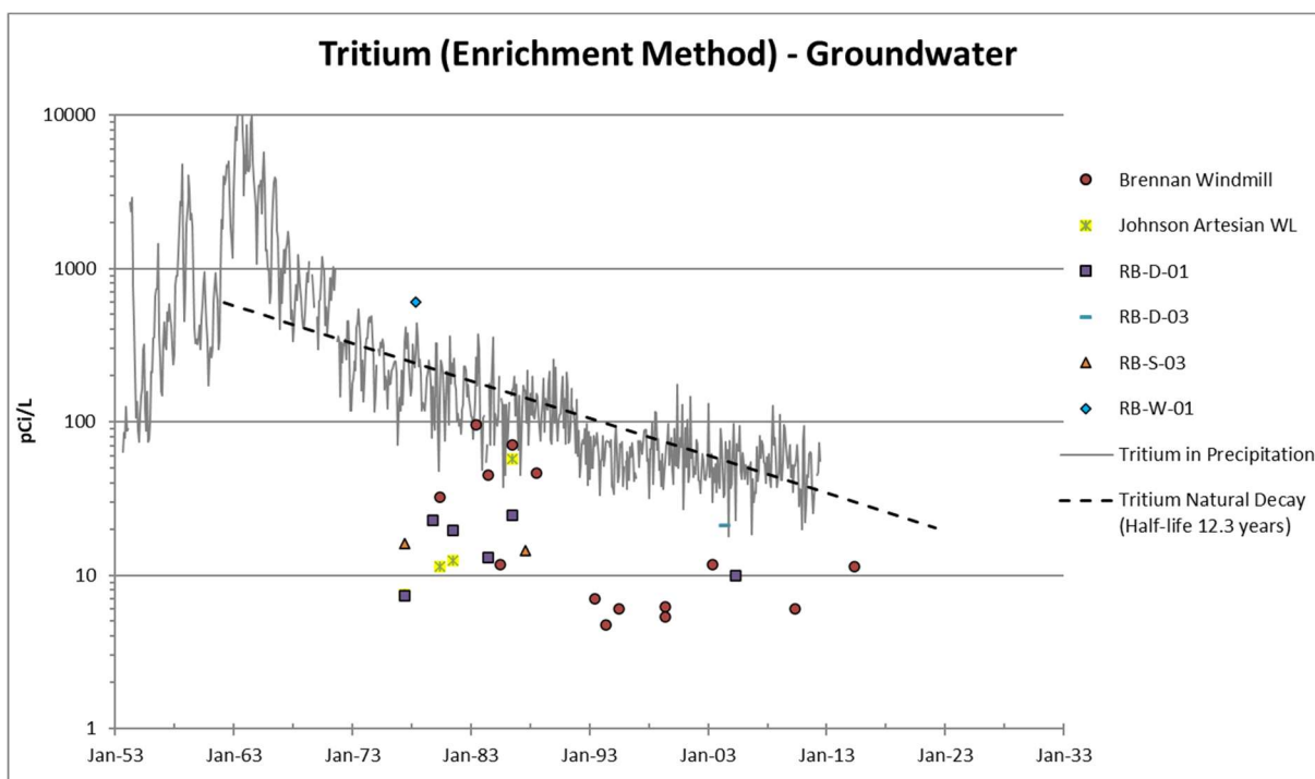
Figure 4. Comparison of Tritium in Wells near the Rio Blanco Site with Tritium in Precipitation at Ottawa, Canada (Site with the Longest Historical Tritium Record [IAEA 2024])
