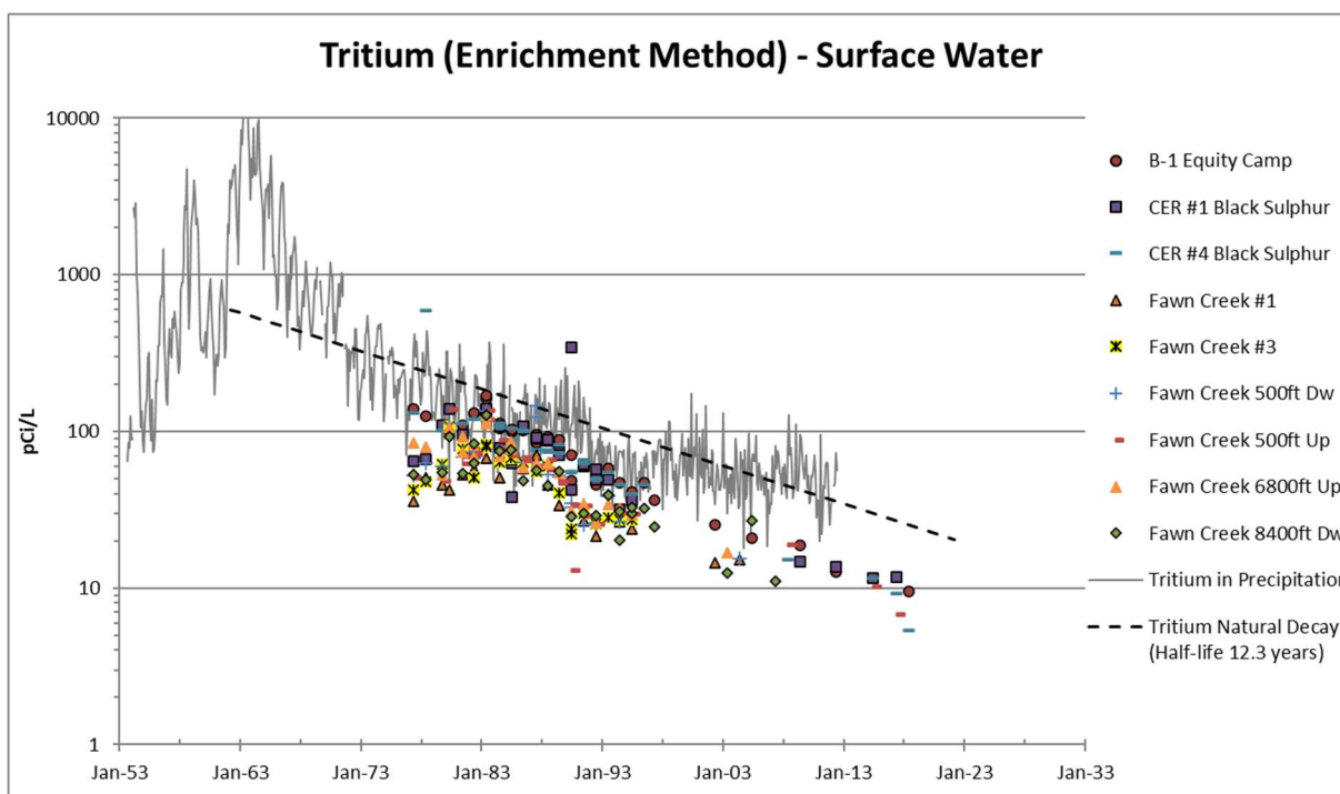
Figure 5. Comparison of Tritium in Surface Water near the Rio Blanco Site with Tritium in Precipitation at Ottawa, Canada (Site with the Longest Historical Tritium Record [IAEA 2024])
