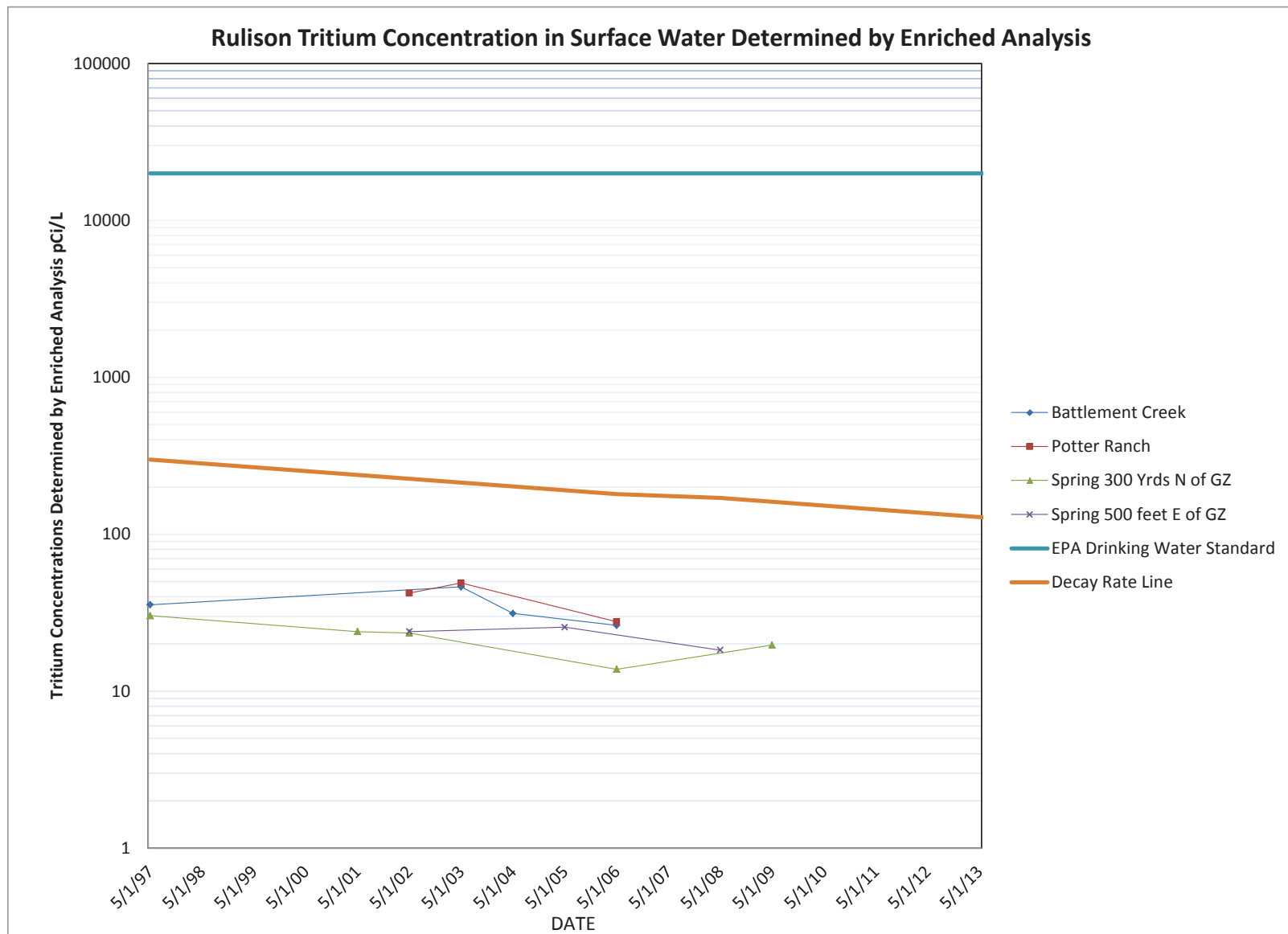
Figure 4. Rulison, Colorado Site, Tritium Concentrations in Surface Water Determined by Enriched Analysis Note: Tritium decay line represents tritium fallout concentrations in precipitation from earlier atmospheric nuclear testing in surface and near-surface ground water Brown, R.M., 1995. Monthly Tritium in Precipitation at Ottawa, Canada 1953–1995, Atomic Energy of Canada Limited, http://www.science.uottawa.ca/~eih/ch7/7tritium.htm
