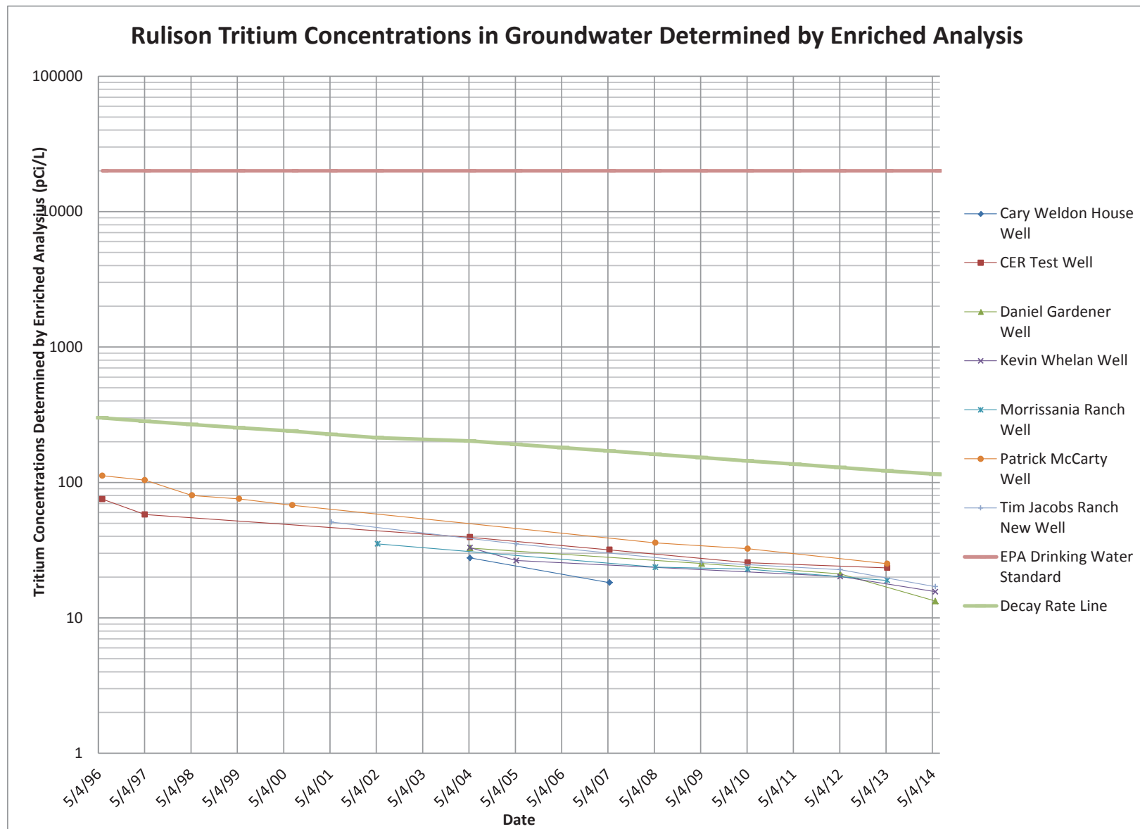
Figure 3. Rulison, Colorado Site, Tritium Concentrations in Groundwater Determined by Enriched Analysis Note: Tritium decay line represents tritium fallout concentrations in precipitation from earlier atmospheric nuclear testing in surface and near-surface ground water Brown, R.M., 1995. Monthly Tritium in Precipitation at Ottawa, Canada 1953–1995, Atomic Energy of Canada Limited, http://www.science.uottawa.ca/~eih/ch7/7tritium.htm
