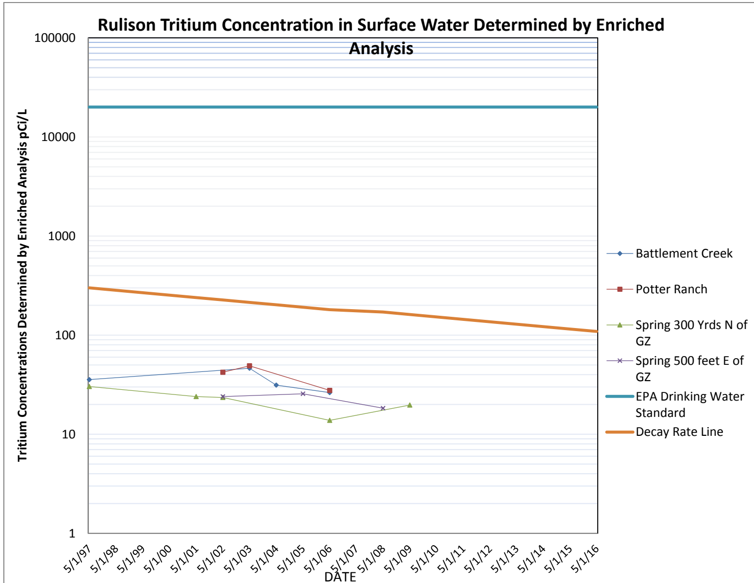
Figure 4. Rulison, Colorado Site, Tritium Concentrations in Surface Water Determined by Enriched Analysis Note: Tritium decay line represents tritium fallout concentrations in precipitation from earlier atmospheric nuclear testing in surface and near-surface ground water (Brown, R.M., 1995. Monthly Tritium in Precipitation at Ottawa, Canada 1953–1995, Atomic Energy of Canada Limited, http://www.science.uottawa.ca/~eih/ch7/7tritium.htm )
