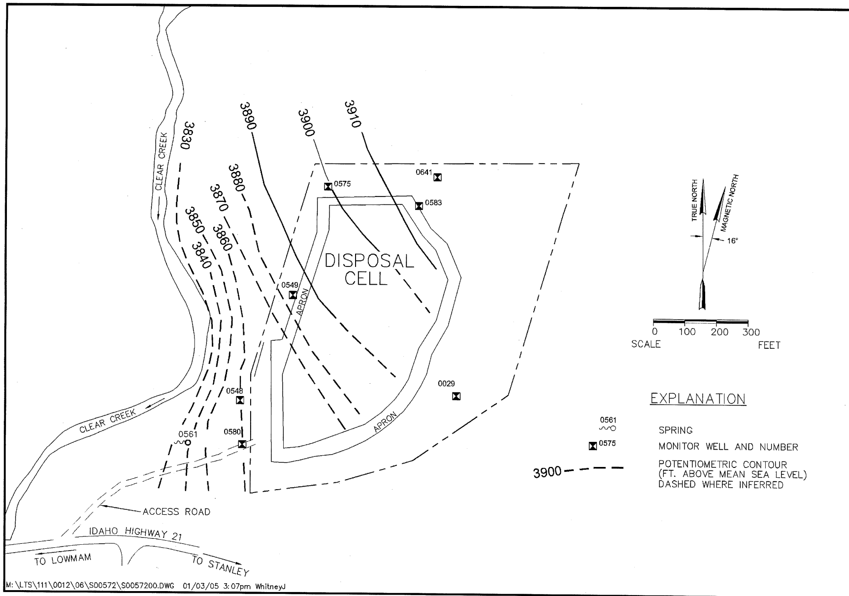
Figure 2-4. Potentiometric Surface at the Lowman, Idaho, Disposal Site
