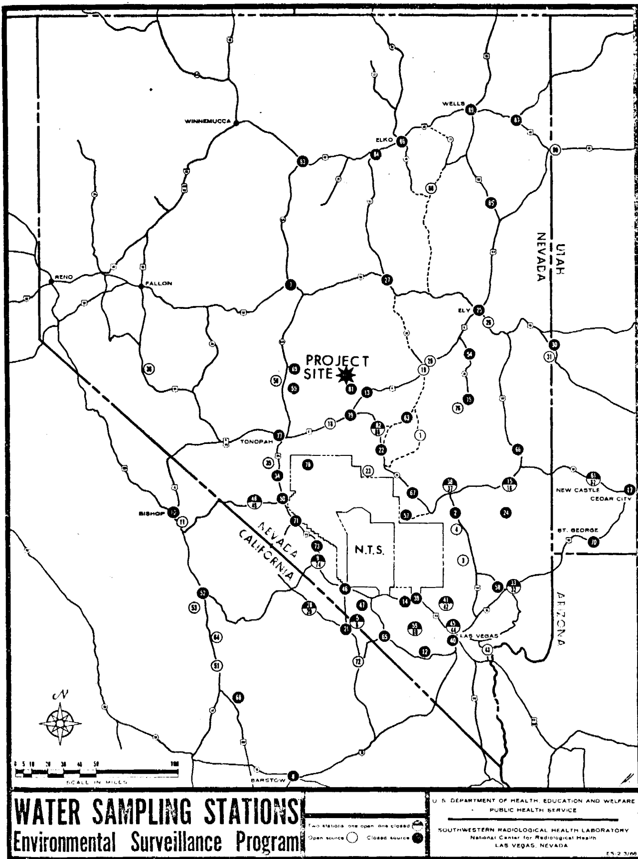
Figure 2. Location of Water Sampling Stations.
