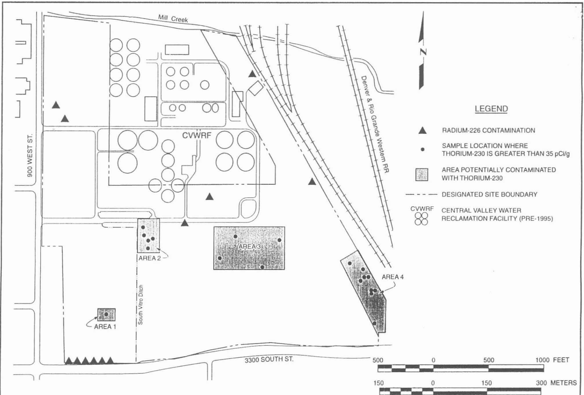
EXHIBIT 2 POST-REMEDIATION RADIOACTIVE CONTAMINATION AREAS SALT LAKE CITY, UTAH, VITRO PROCESSING SITE
