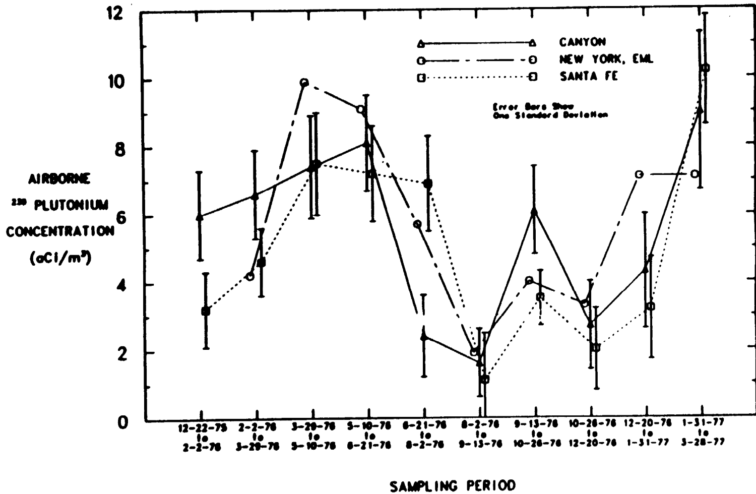
Fig. 11. Concentrations of airborne ^{239}\text{Pu} at three locations during 1976-1977.
