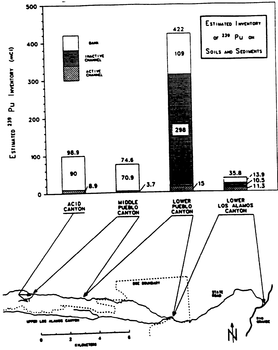
Fig. 10. Estimated inventory of 239 Pu on soils and sediments by location.
