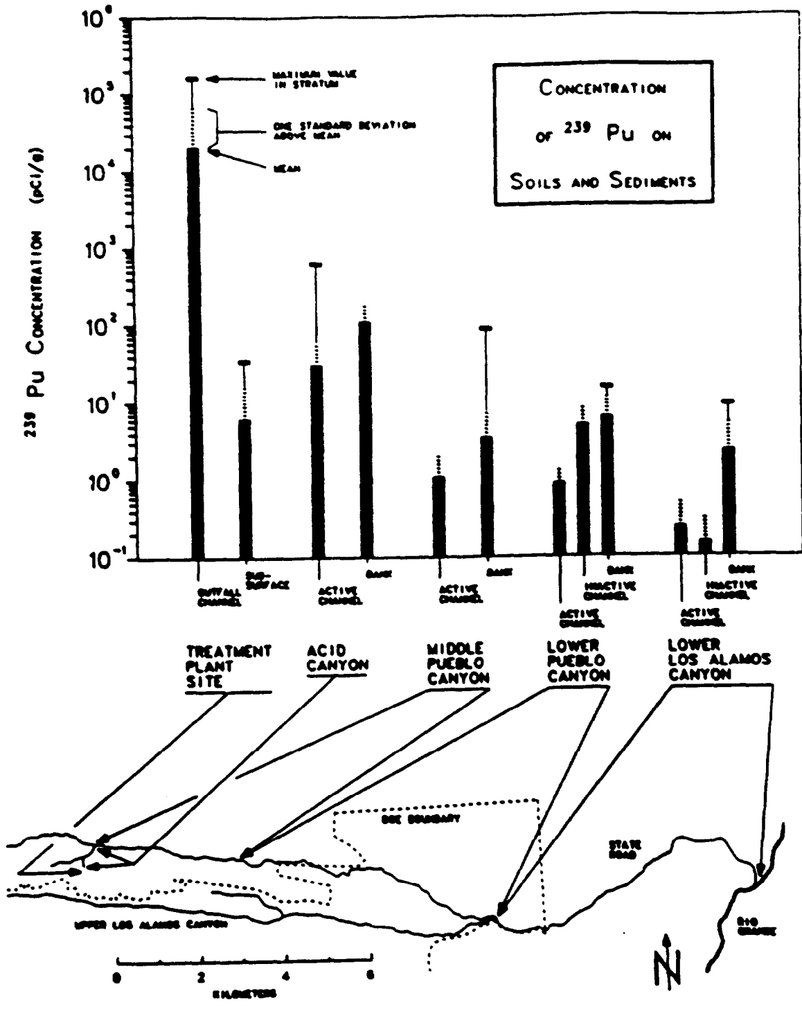
Fig. 9. Concentration of ^{239}\text{Pu} on soils and sediments by location.
