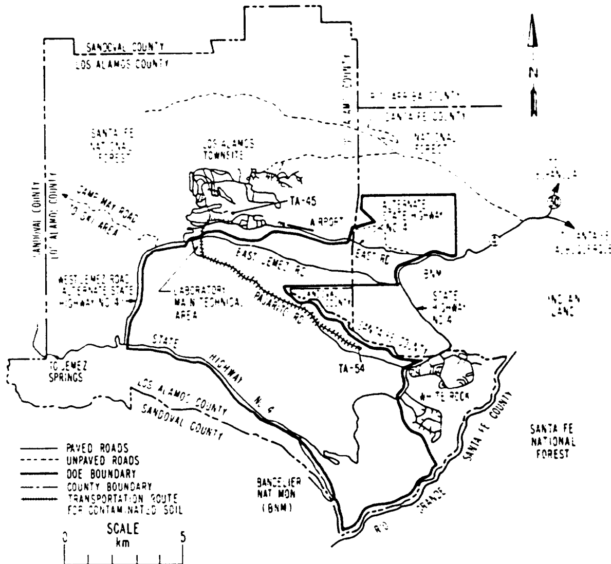
Fig. 7. Location of TA-54 and transportation route from former TA-45 site.
