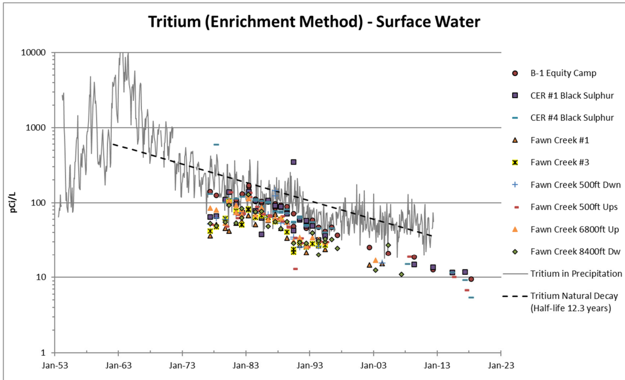
Figure 5. Comparison of Tritium in Surface Water near the Rio Blanco Site with Tritium in Precipitation at Ottawa, Canada (Site with Longest Historical Tritium Record [IAEA 2023])
