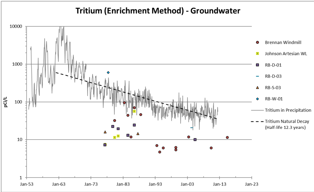
Figure 4. Comparison of Tritium in Wells near the Rio Blanco Site with Tritium in Precipitation at Ottawa, Canada (Site with Longest Historical Tritium Record [IAEA 2023])
