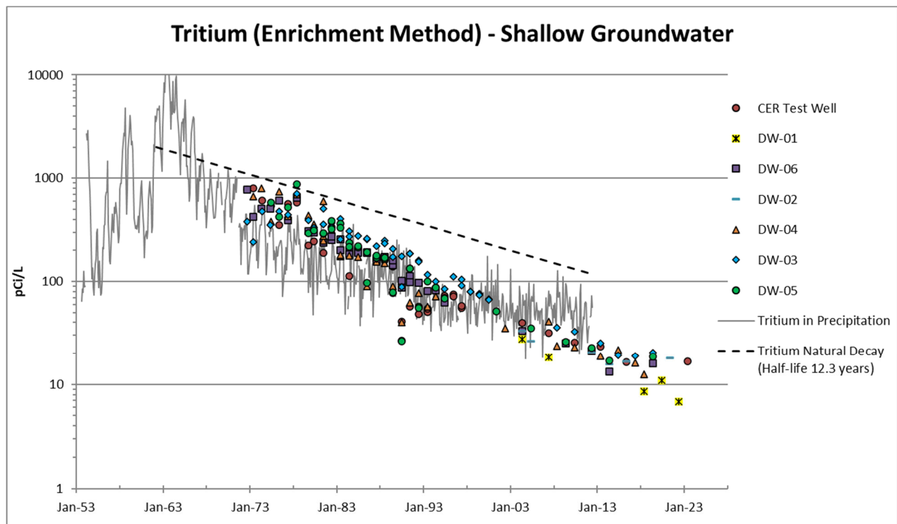
Figure 5. Comparison of Tritium in Shallow Wells near the Rulison Site with Tritium in Precipitation at Ottawa, Canada (Site with Longest Historical Tritium Record [IAEA 2022])
