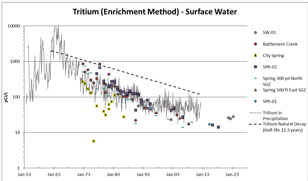
Figure 6. Comparison of Tritium in Surface Water near the Rulison Site with Tritium in Precipitation at Ottawa, Canada (Site with Longest Historical Tritium Record [IAEA 2022])
