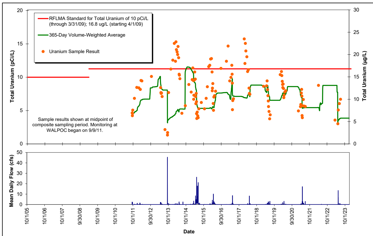
Figure 51. Composite Sample Uranium Results and Rolling 365-Day Averages at WALPOC: Postclosure
