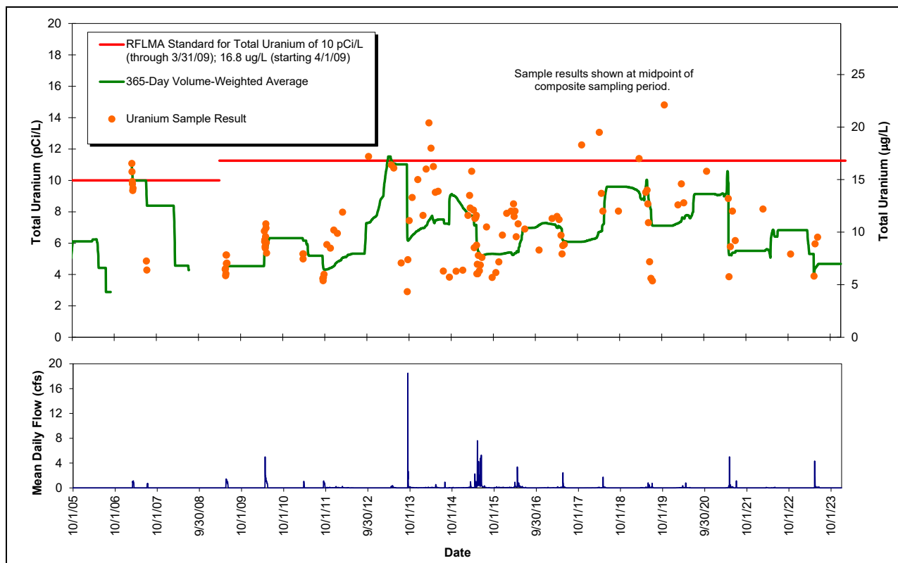
Figure 41. Composite Sample Uranium Results and Rolling 365-Day Averages at GS08: Postclosure
