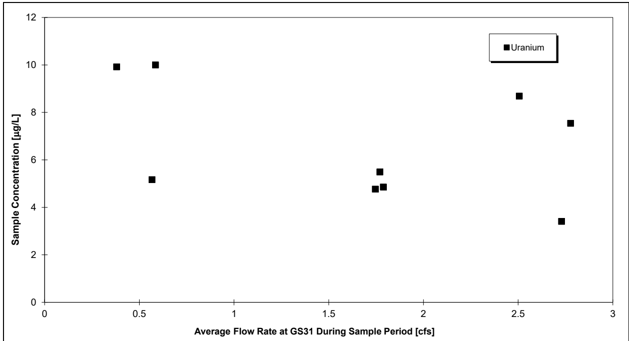
Figure 32. Uranium Concentrations Versus Average Sample Flow Rate for GS31 Storm-Event Samples
