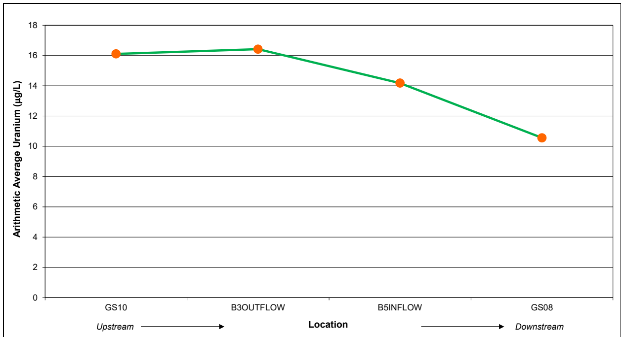
Figure 54. Arithmetic Average Uranium Concentrations at South Walnut Creek Grab Locations
