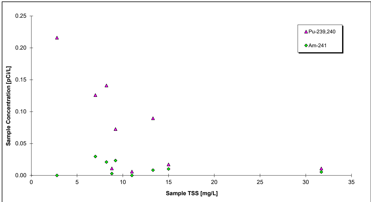
Figure 30. Plutonium and Americium Concentrations Versus Total Suspended Solids for GS31 Storm-Event Samples
