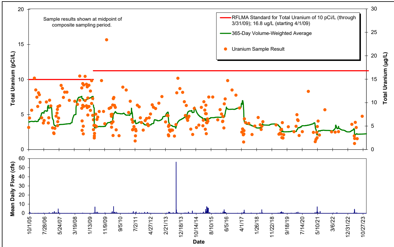
Figure 43. Composite Sample Uranium Results and Rolling 365-Day Averages at SW093: Postclosure
