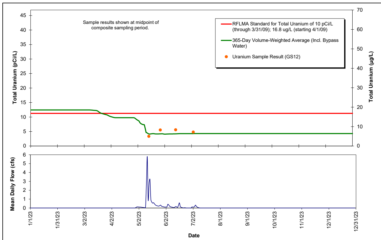
Figure 46. Composite Sample Uranium Results and Rolling 365-Day Averages at GS12: CY 2023
