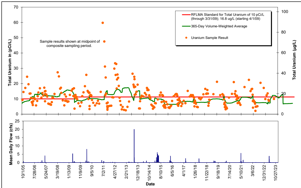
Figure 37. Composite Sample Uranium Results and Rolling 365-Day Averages at GS10: Postclosure
