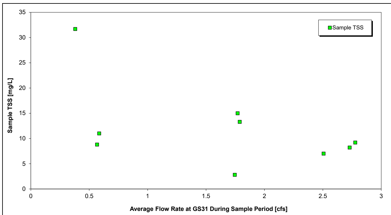
Figure 33. Total Suspended Solids Versus Average Sample Flow Rate for GS31 Storm-Event Samples
