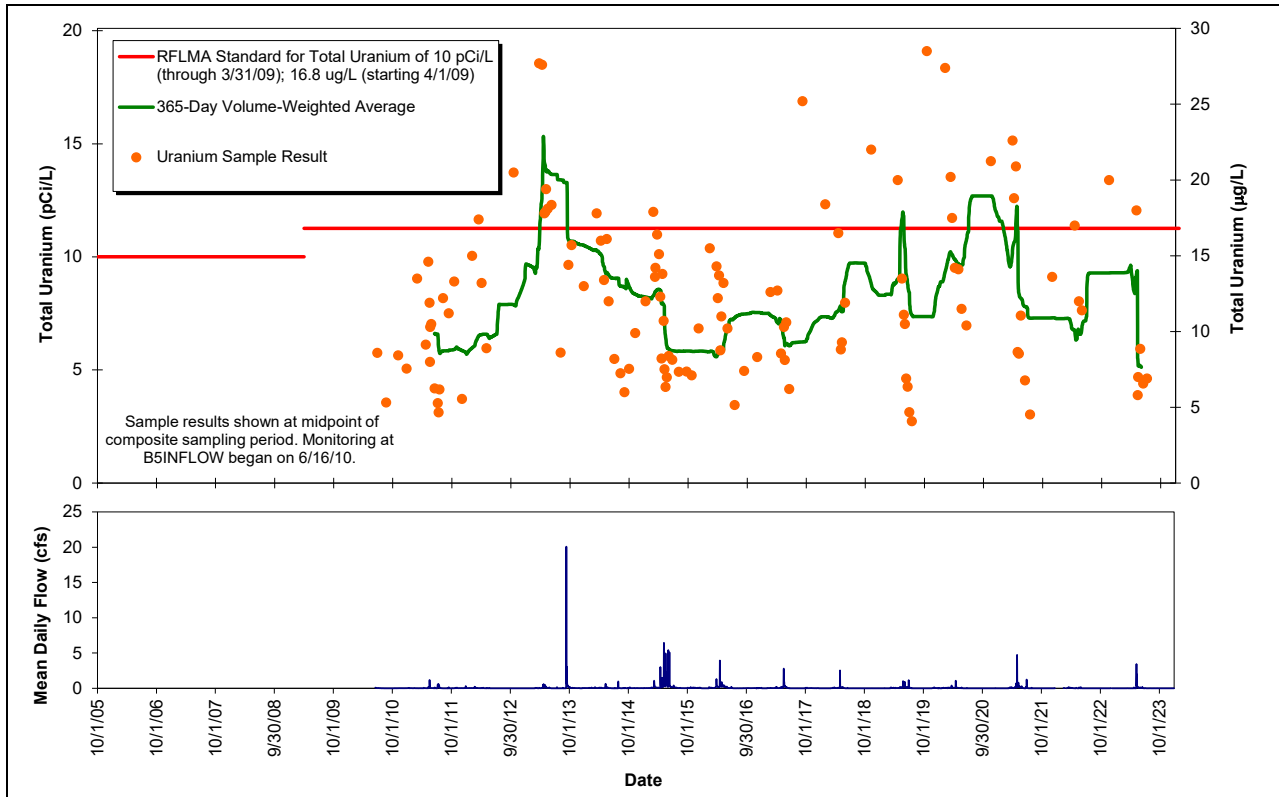
Figure 39. Composite Sample Uranium Results and Rolling 365-Day Averages at B5INFLOW: Postclosure
