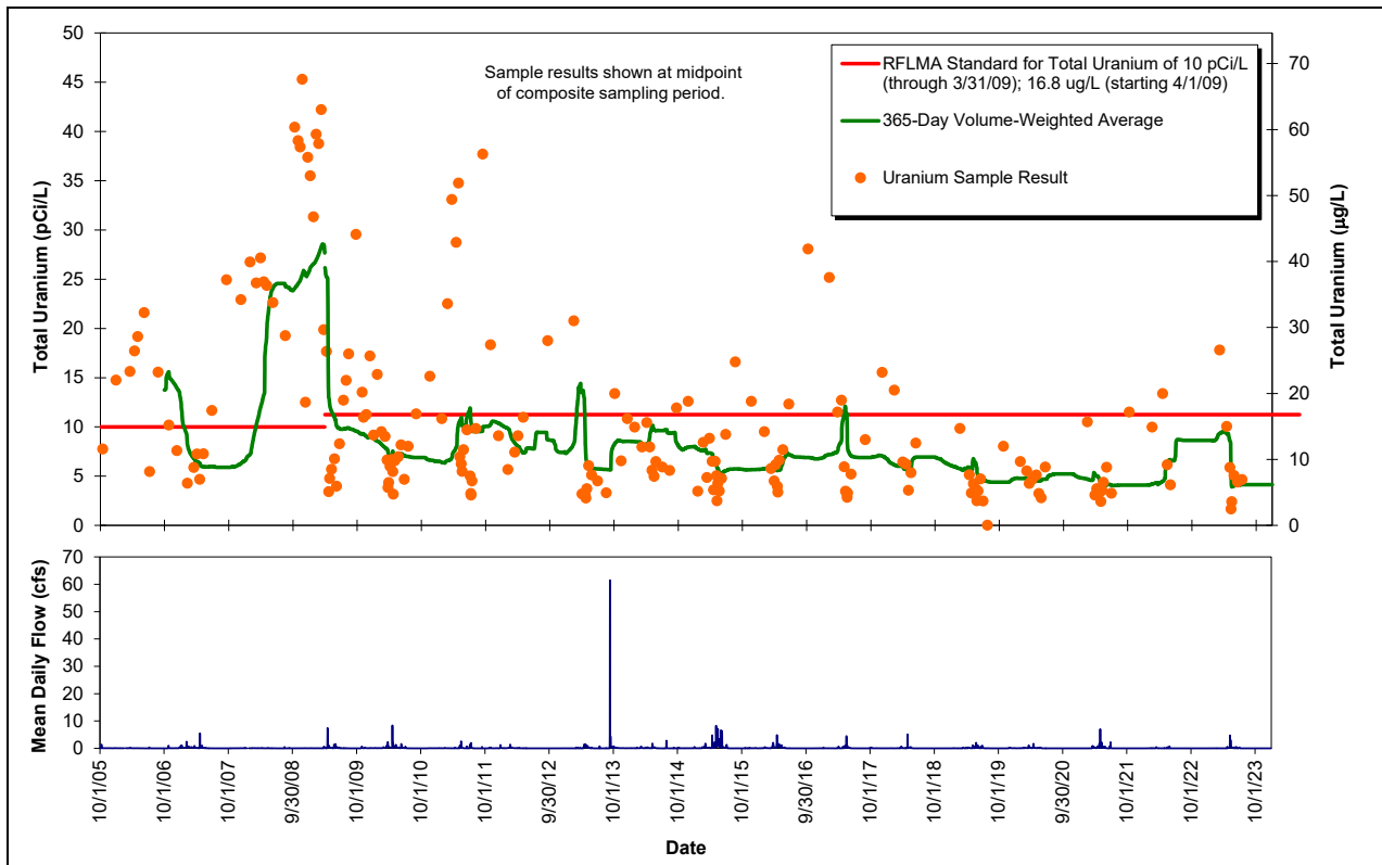
Figure 45. Composite Sample Uranium Results and Rolling 365-Day Averages at GS13: Postclosure
