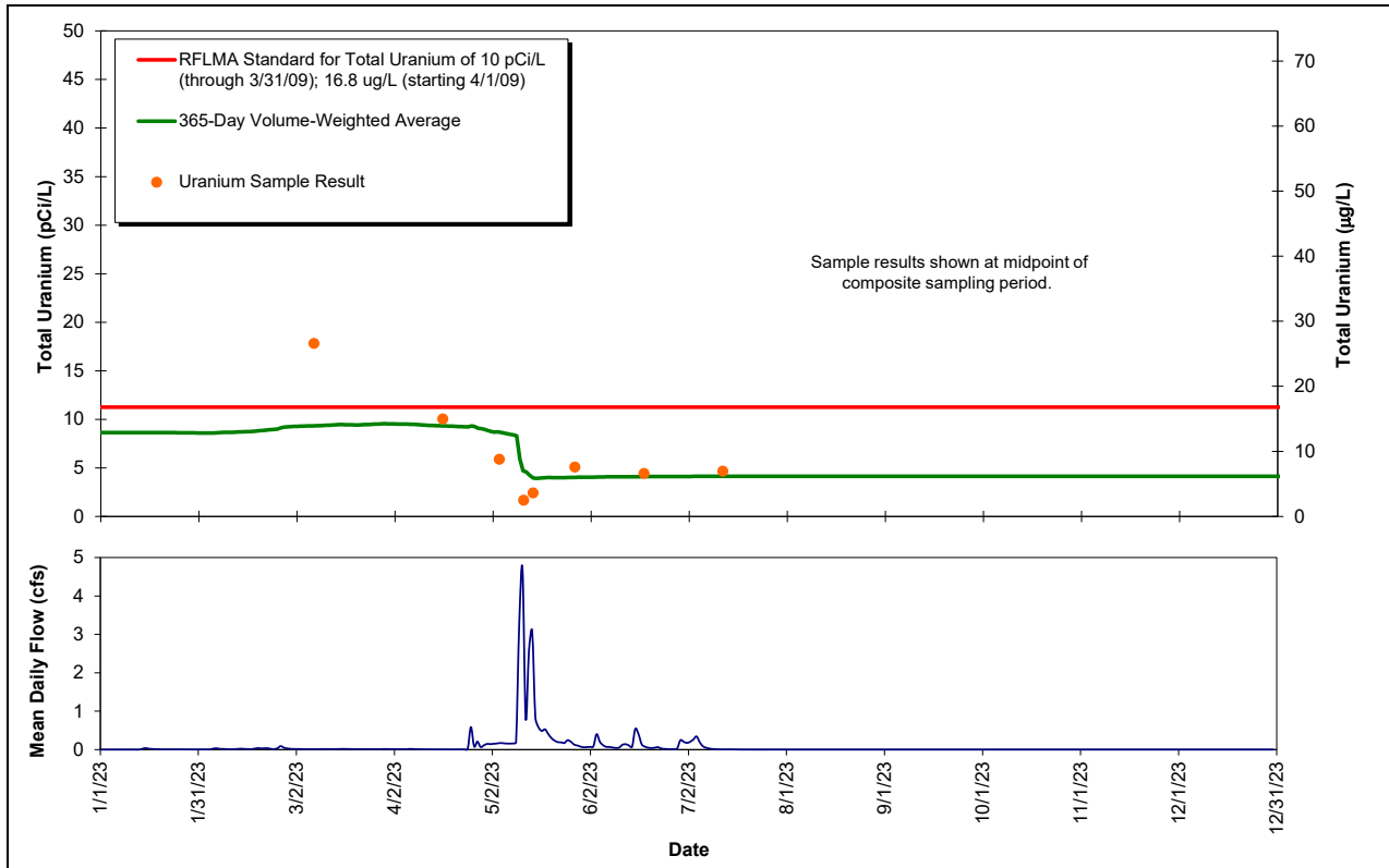
Figure 44. Composite Sample Uranium Results and Rolling 365-Day Averages at GS13: CY 2023
