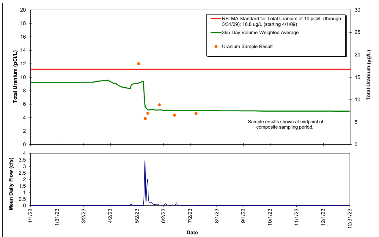
Figure 38. Composite Sample Uranium Results and Rolling 365-Day Averages at B5INFLOW: CY 2023
