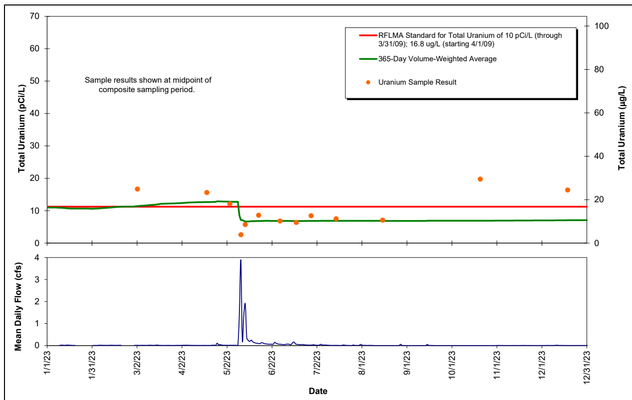
Figure 36. Composite Sample Uranium Results and Rolling 365-Day Averages at GS10: CY 2023
