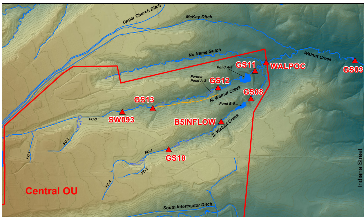
Figure 34. Continuous Flow-Paced Composite Sampling Locations in Walnut Creek
