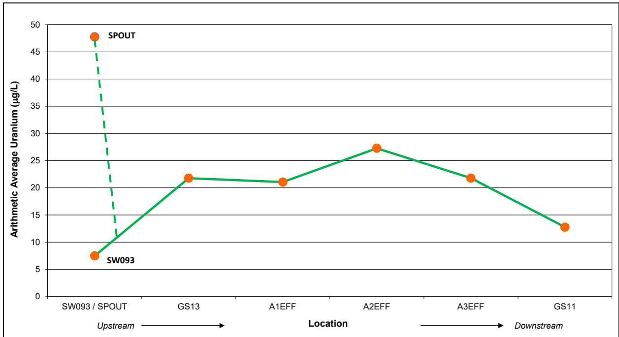
Figure 53. Arithmetic Average Uranium Concentrations at North Walnut Creek Grab Locations
