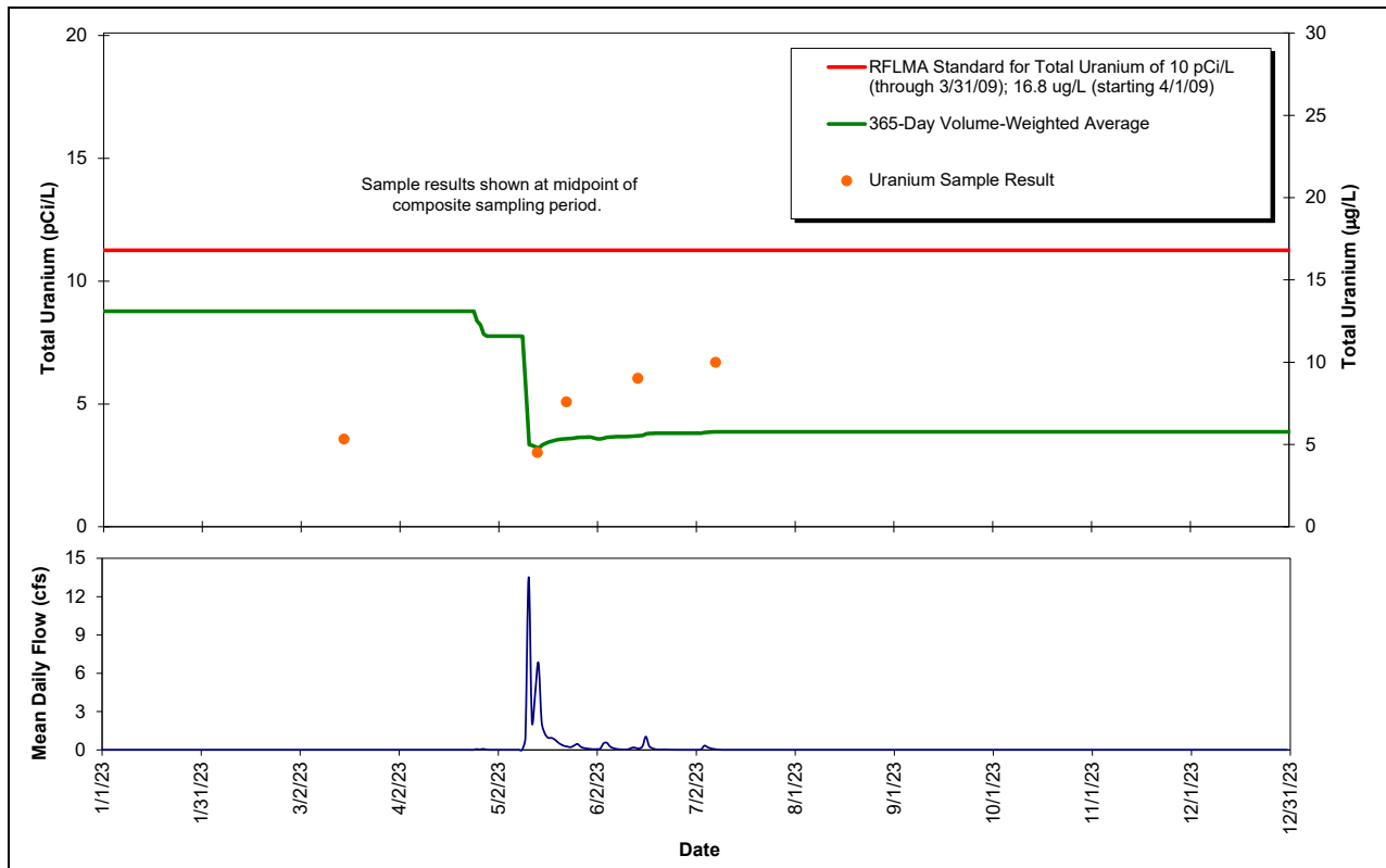
Figure 50. Composite Sample Uranium Results and Rolling 365-Day Averages at WALPOC: CY 2023
