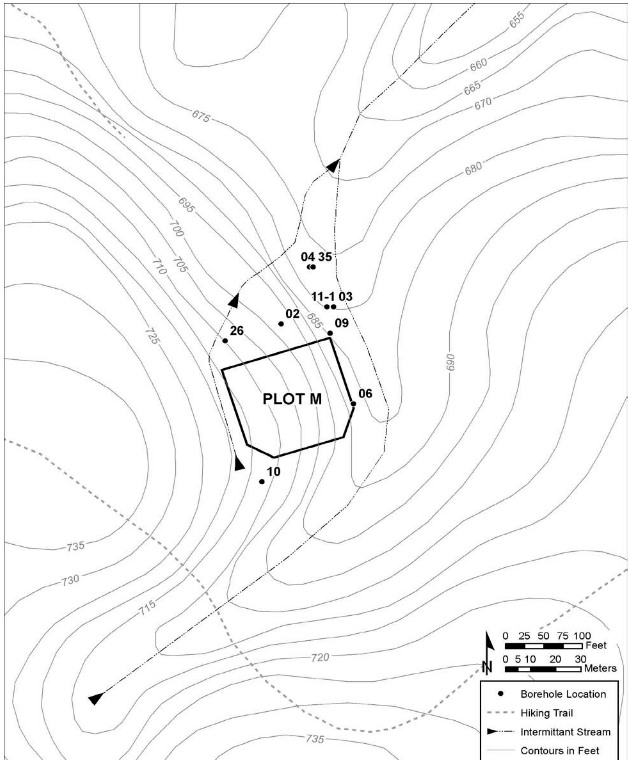
Figure 3.2 Map of Plot M Palos Site Showing Topography, Intermittent Stream, and Monitoring Well Locations
