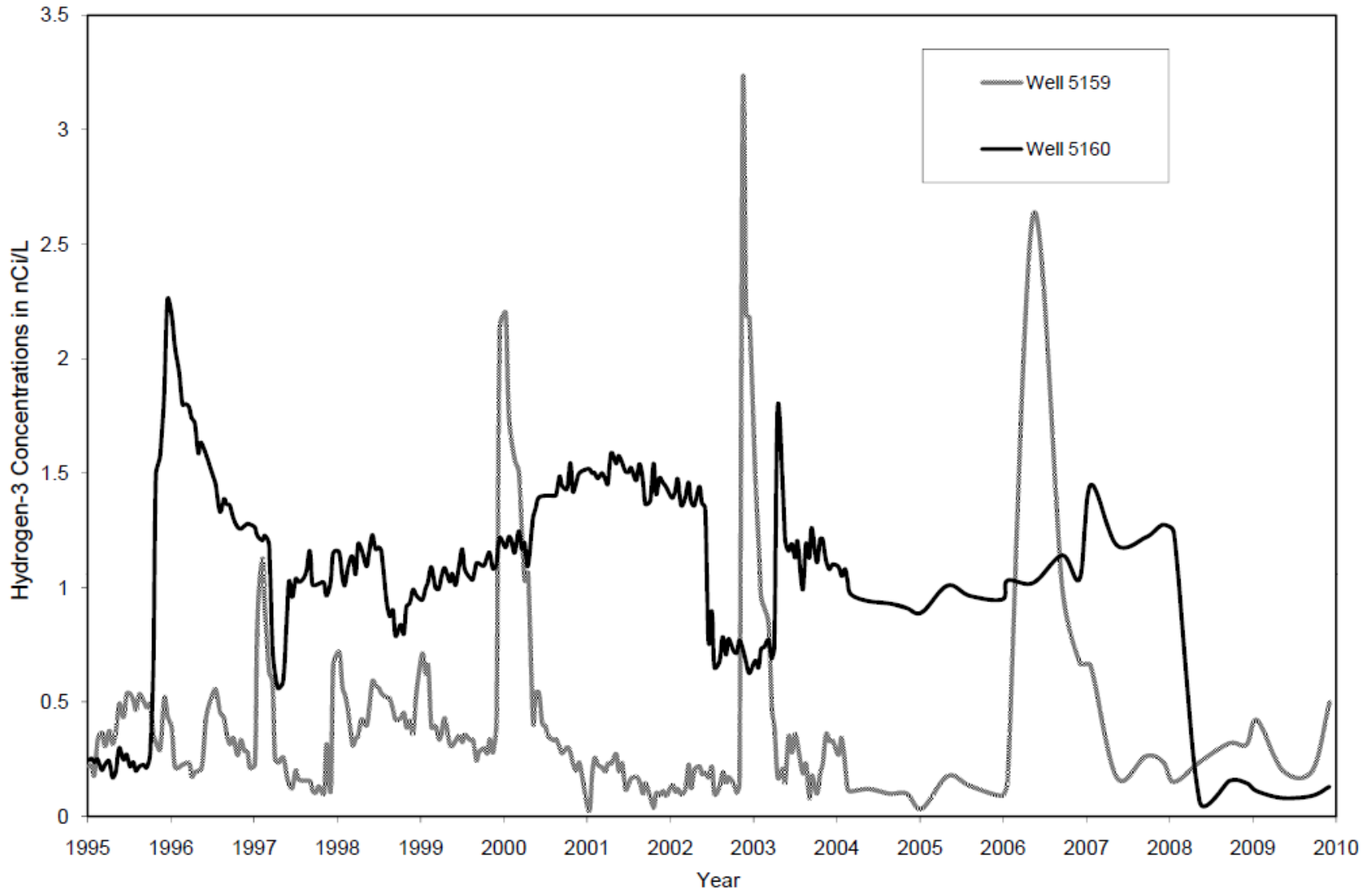
Figure 3.5 Hydrogen-3 Concentrations in Opposite Red Gate Woods (#5159) and Red Gate Woods North (#5160) Wells From 1995 Through 2009
