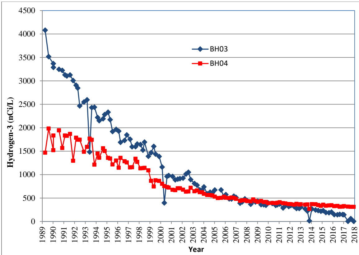
Figure 4.3 Hydrogen-3 in Plot M Wells BH03 and BH04
