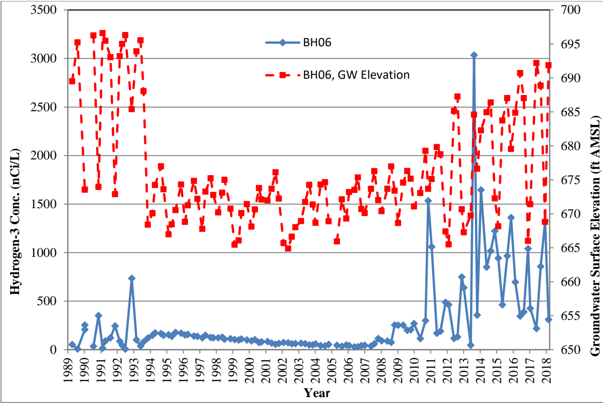
Figure 4.5 Hydrogen-3 and Groundwater Elevation in Well BH06
