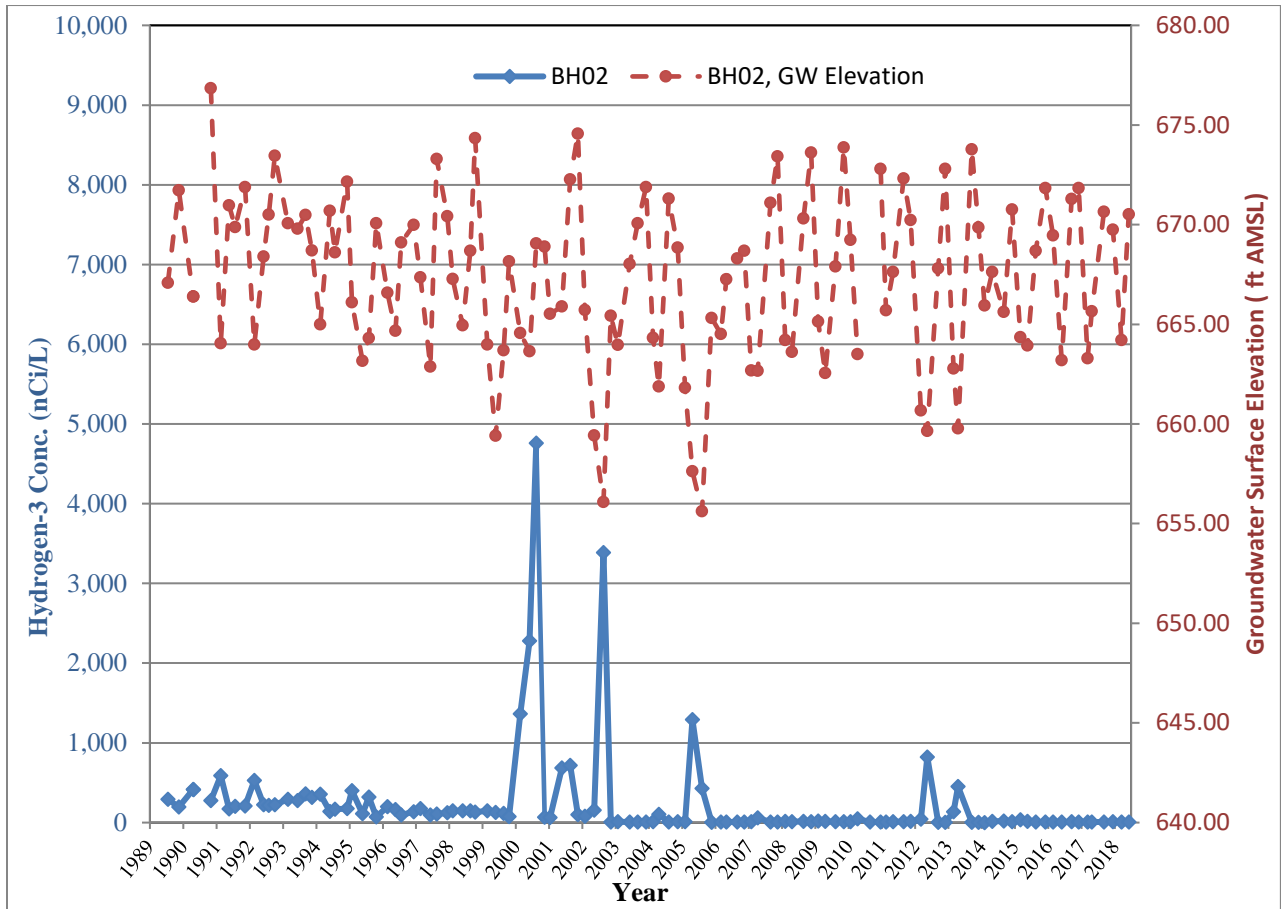
Figure 4.7 Hydrogen-3 and Groundwater Elevation in Well BH02
