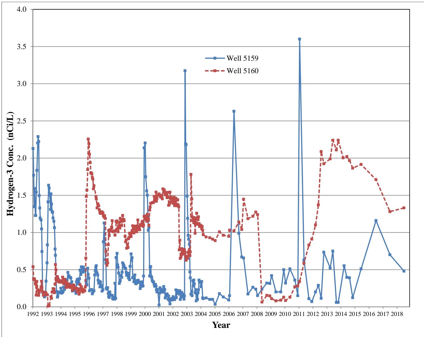
Figure 4.12 Hydrogen-3 in Former Picnic Wells from 1992 Through 2018
