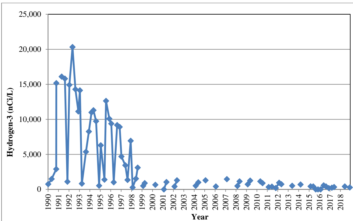
Figure 4.4 Hydrogen-3 in Plot M Well BH09
