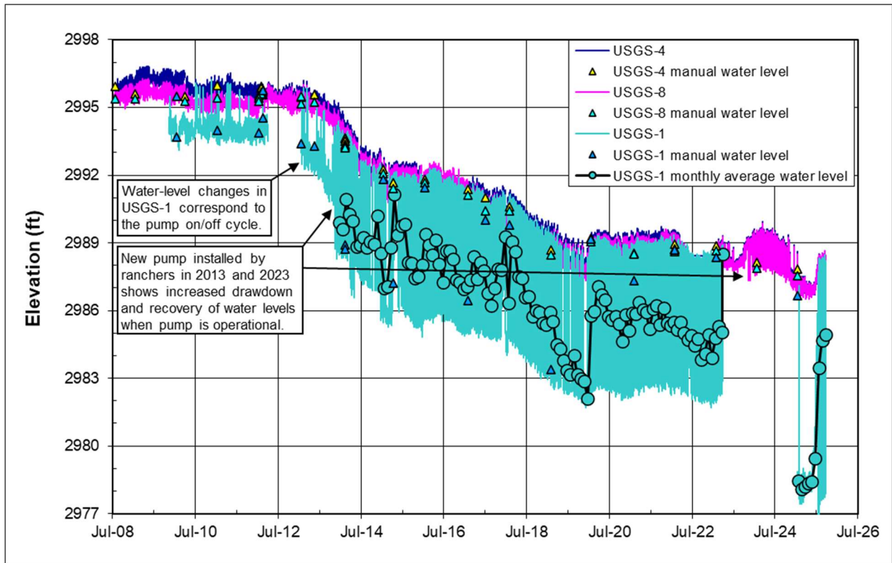
Figure 6. Groundwater Elevations in Culebra Wells, 2008 Through September 2025
