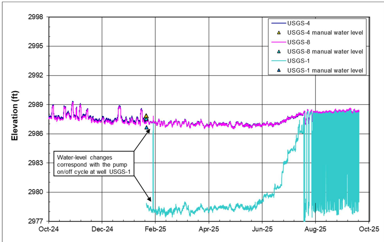
Figure 7. Groundwater Elevations in Culebra Wells, 2025 Reporting Period
