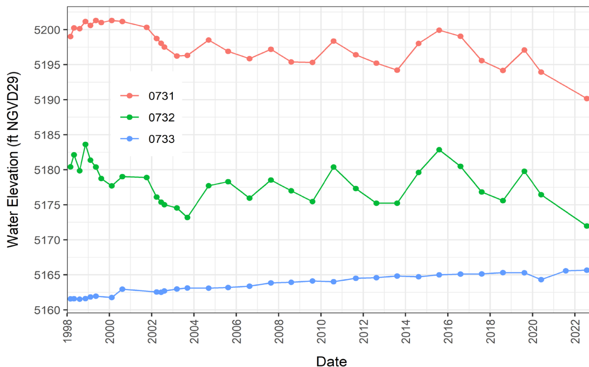
Figure 6-3. Water Level Measurements at the Grand Junction, Colorado, Disposal Site
