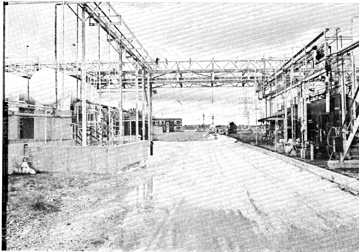
Fig. 6. Southern view of the overhead pipe rack system between the buildings on the left and the spill containment area on the right at Uniroyal Chemical Company, 720 Fairport-Nursery Road, Painesville, Ohio (DMP001).
