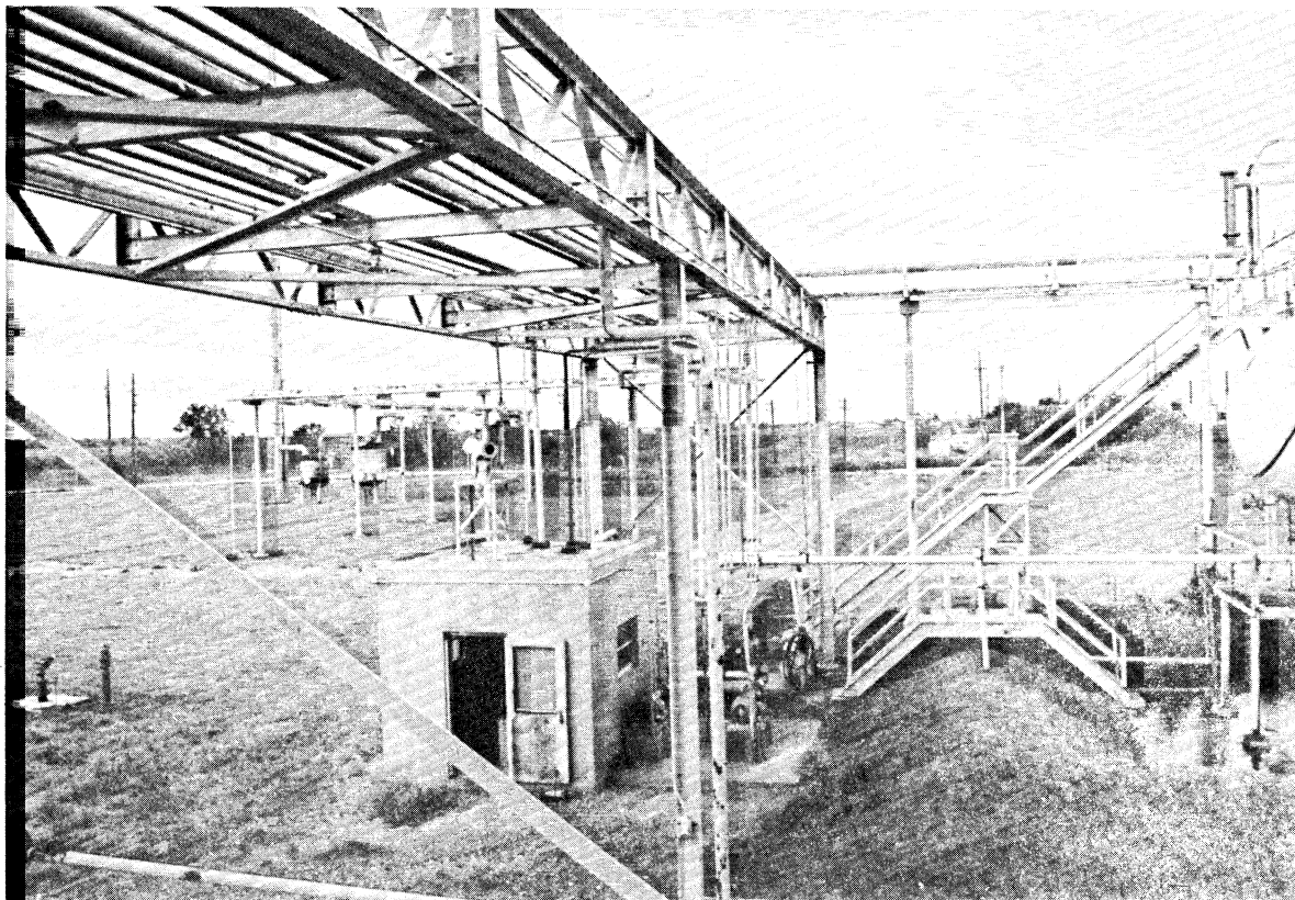
Fig. 5. Western view of the property, showing the overhead pipe rack system from the southern end of the butadiene storage tank at Uniroyal Chemical Company, 720 Fairport-Nursery Road, Painesville, Ohio (DMP001).
