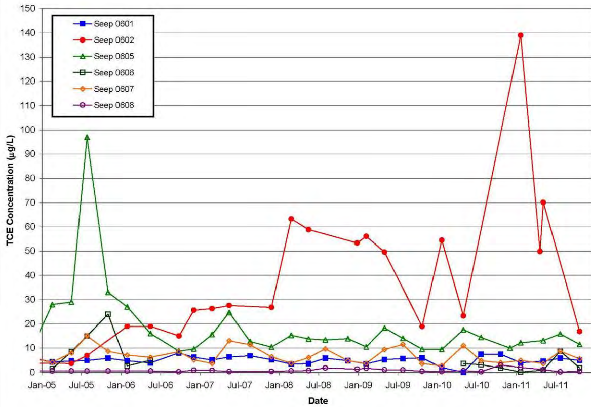
Figure 5. TCE Concentrations in the Main Hill Seeps (2005–2011)
