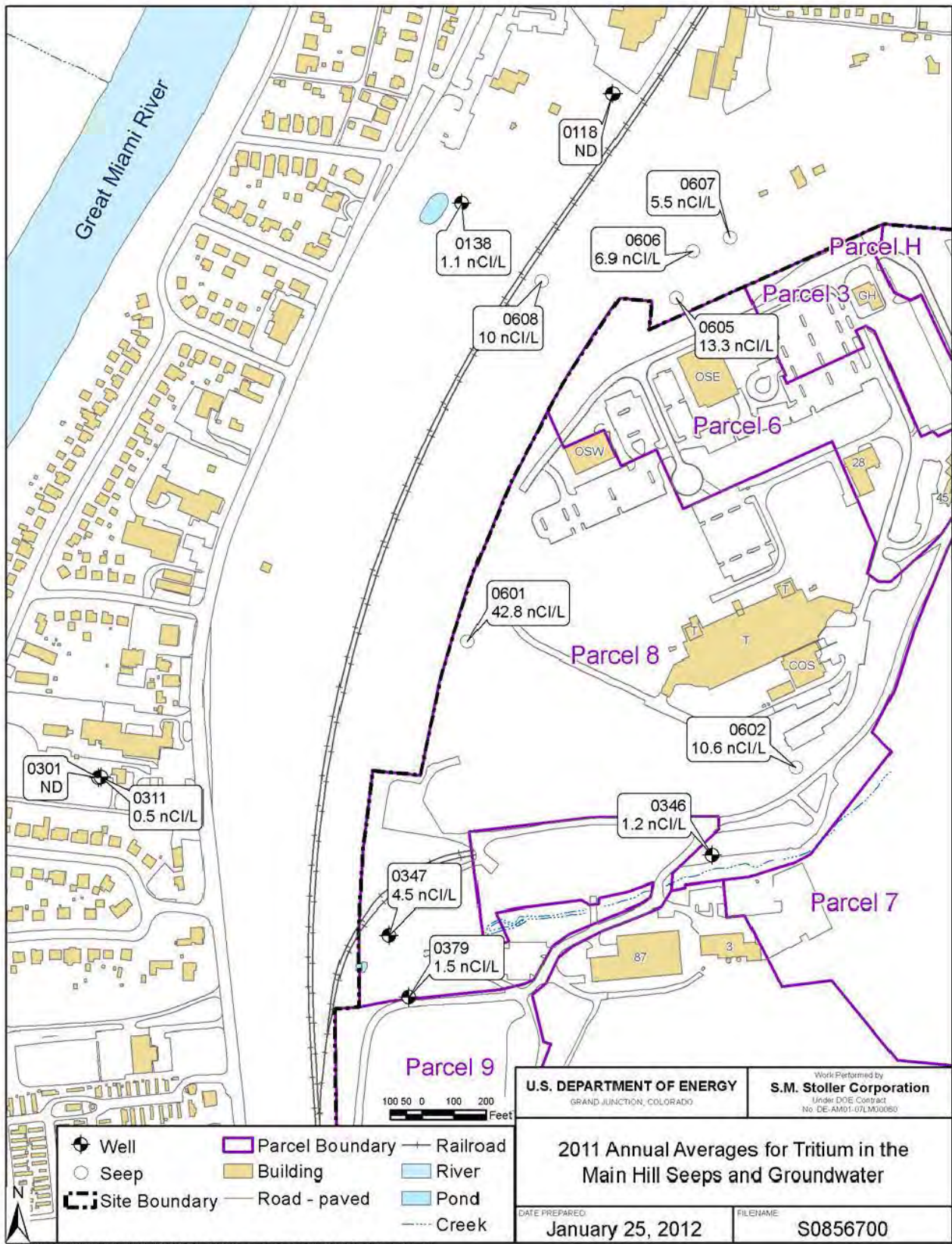
Figure 11. 2011 Annual Average Tritium Levels in the Main Hill Seeps
