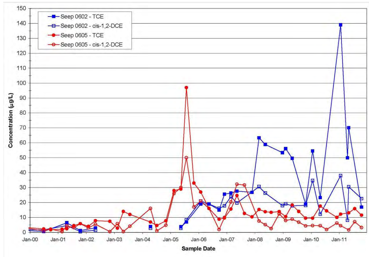
Figure 7. TCE and cis -1,2-DCE Concentrations in Seeps 0602 and 0605 (2000–2011)
