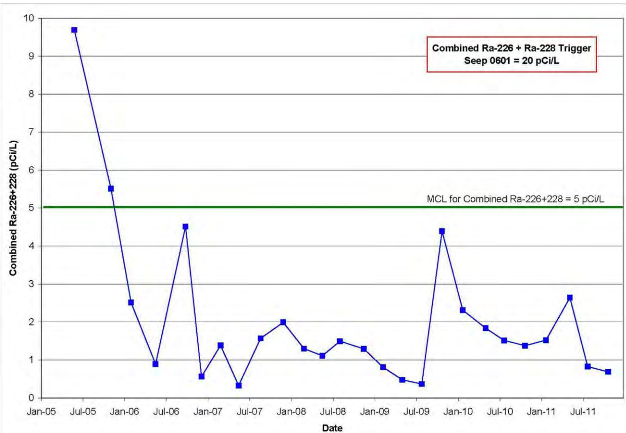
Figure 13. Combined Ra-226/228 Activity over Time in Seep 0601 (2005–2011)
