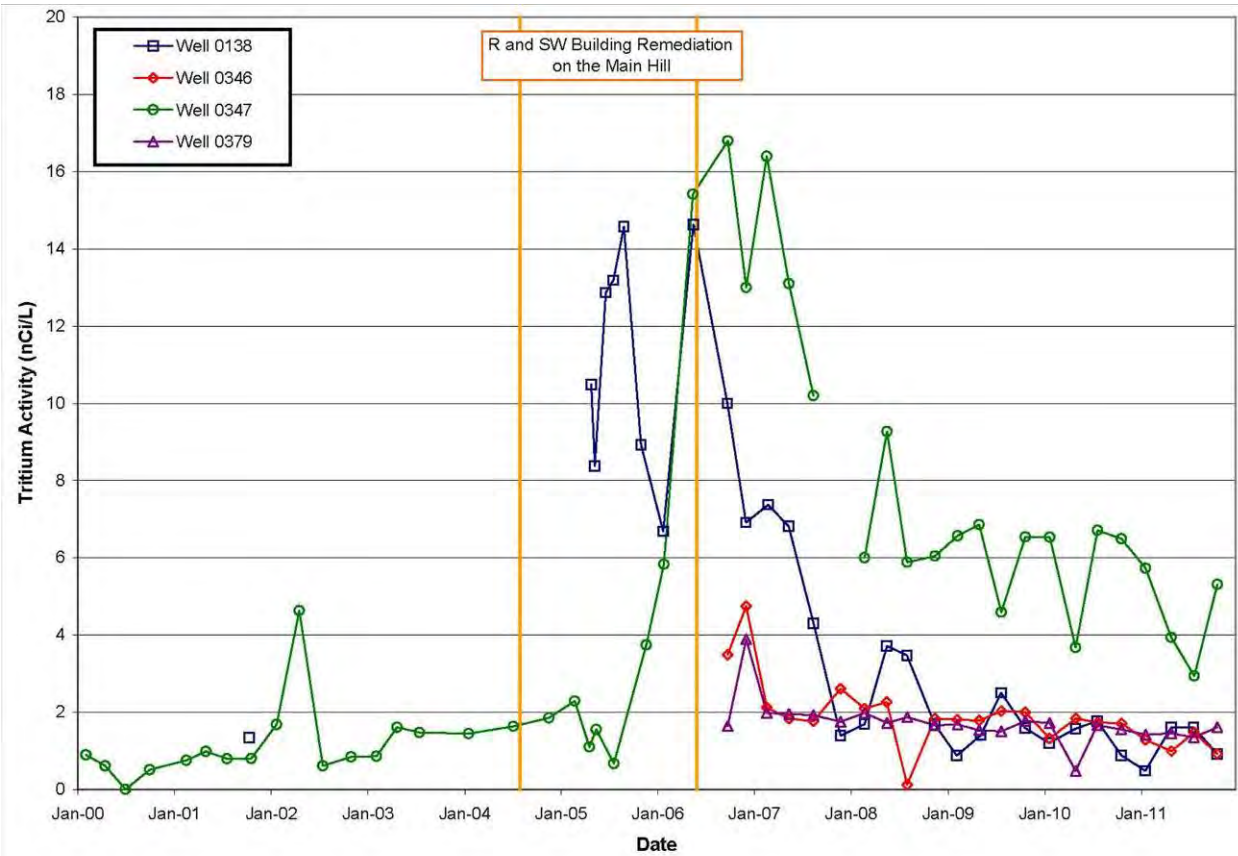
Figure 10. Tritium Activity in Wells 0138, 0346, 0347, and 0379 (2000–2011)
