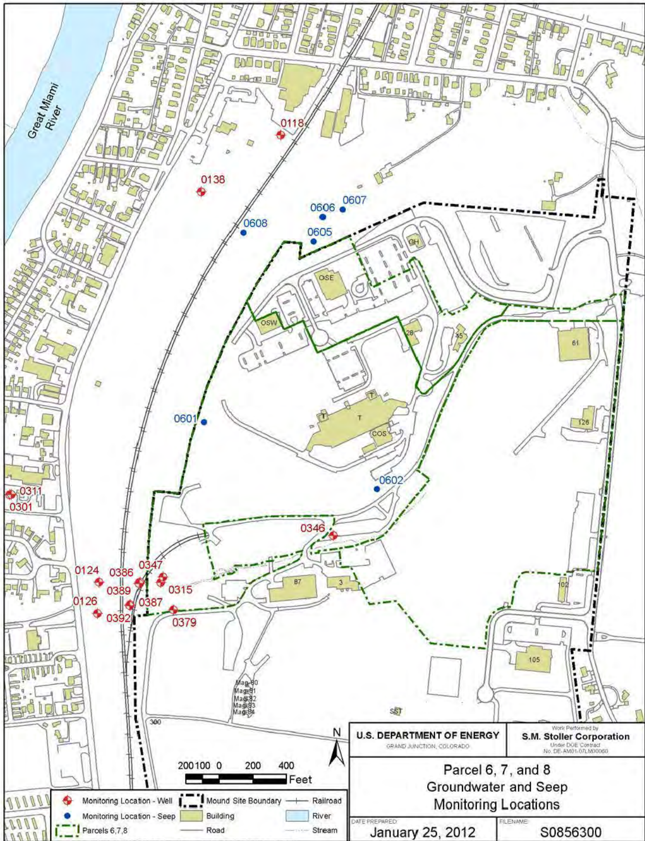
Figure 1. Parcel 6, 7, and 8 Groundwater and Seep Monitoring Locations
