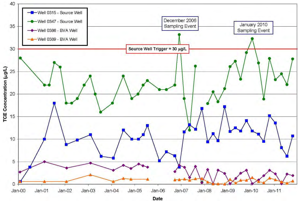
Figure 3. TCE Concentrations in Well 0315/0347 Area (2000–2011)
