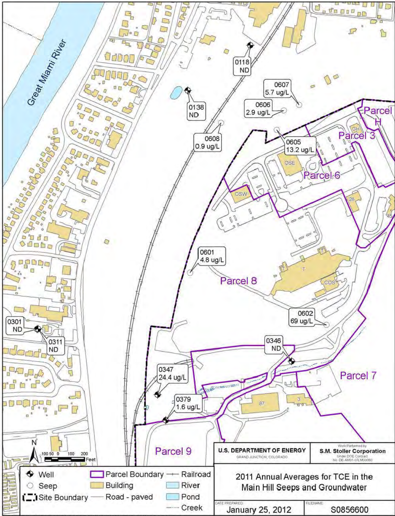
Figure 8. 2011 Annual Average TCE Concentrations in the Main Hill Seeps
