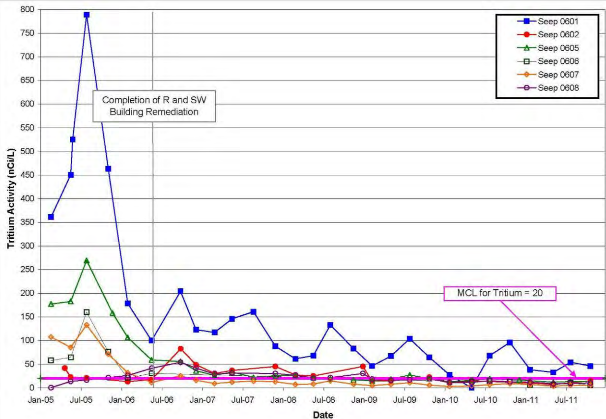
Figure 9. Tritium Activity in Seeps (2005–2011)
