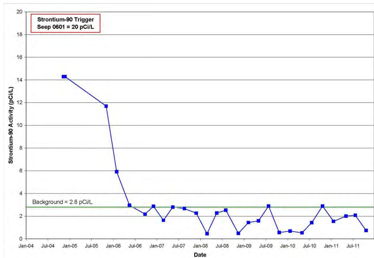
Figure 12. Sr-90 Activity over Time in Seep 0601 (2004–2011)
