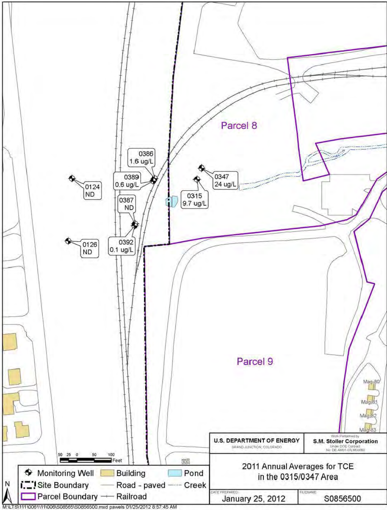
Figure 4. 2011 Annual Average TCE Concentrations in Well 0315/0347 Area
