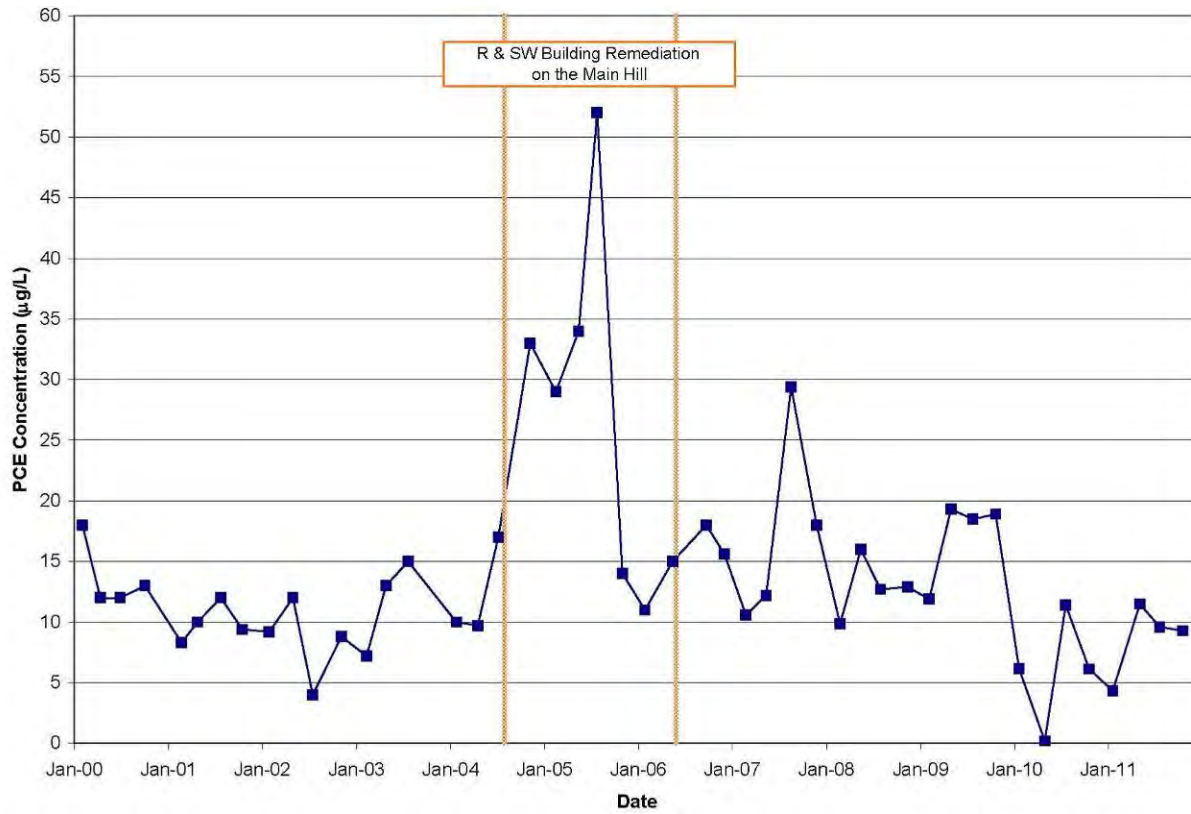
Figure 6. PCE Concentrations in Seep 0601 (2000–2011)
