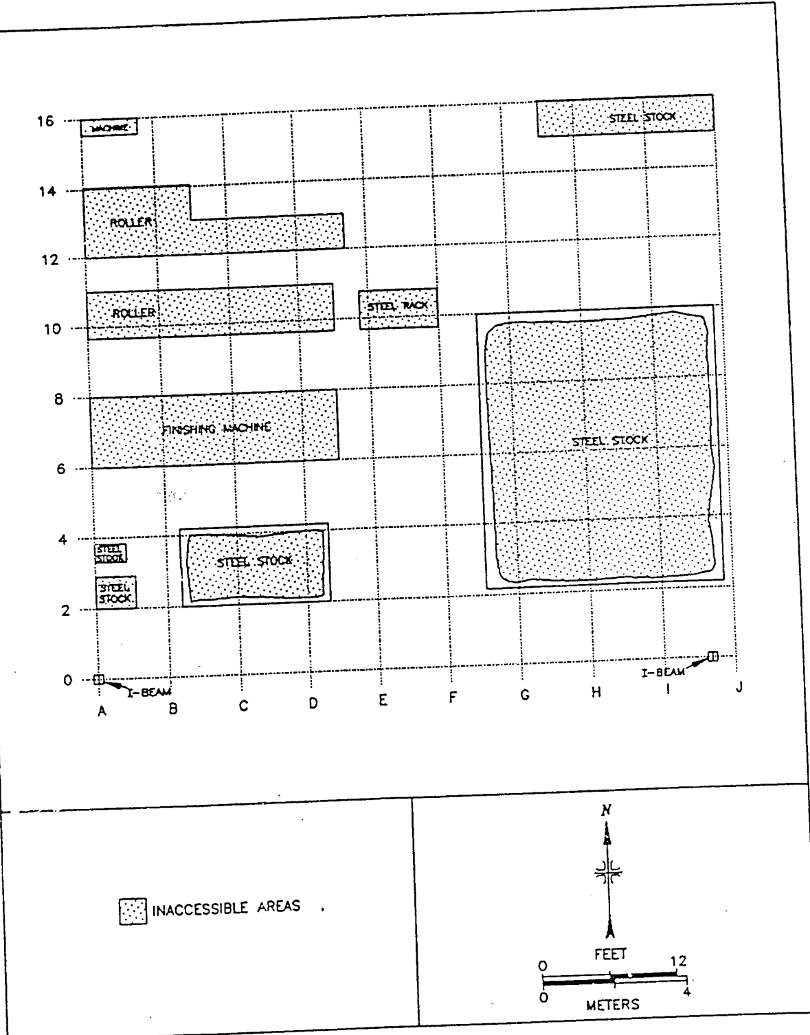
FIGURE 3: "Special Finishing" Area - Floor Plan and Reference Grid
