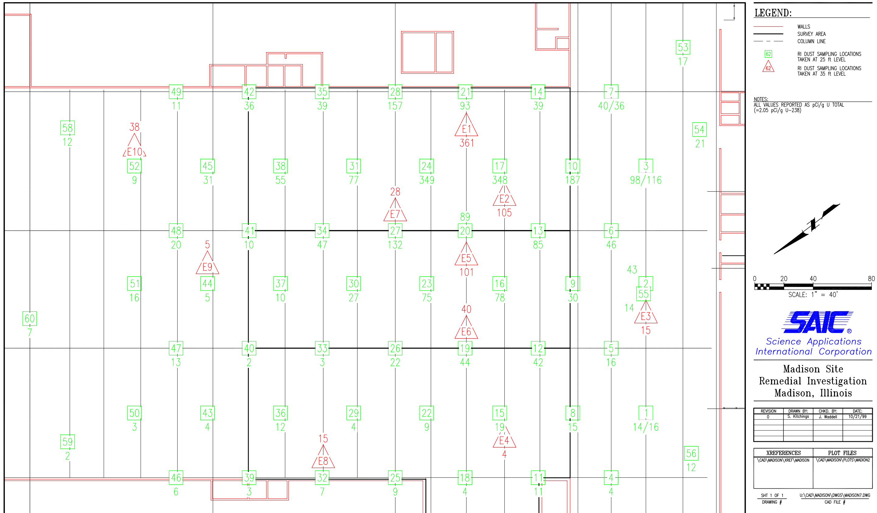
Figure 2. Diagram of Southwest portion of Building 6, indicating locations of dust sampling from major overhead beams in the vicinity of the Extrusion Press.
