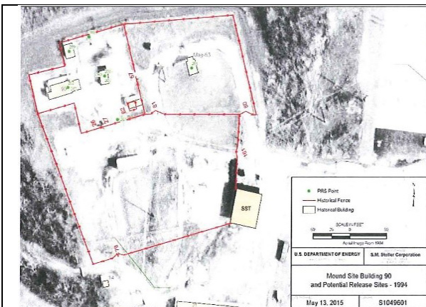
Figure 7. Diagram of RCRA Burn Area Boundary (Salt Shed Is Not Within the Boundary)
