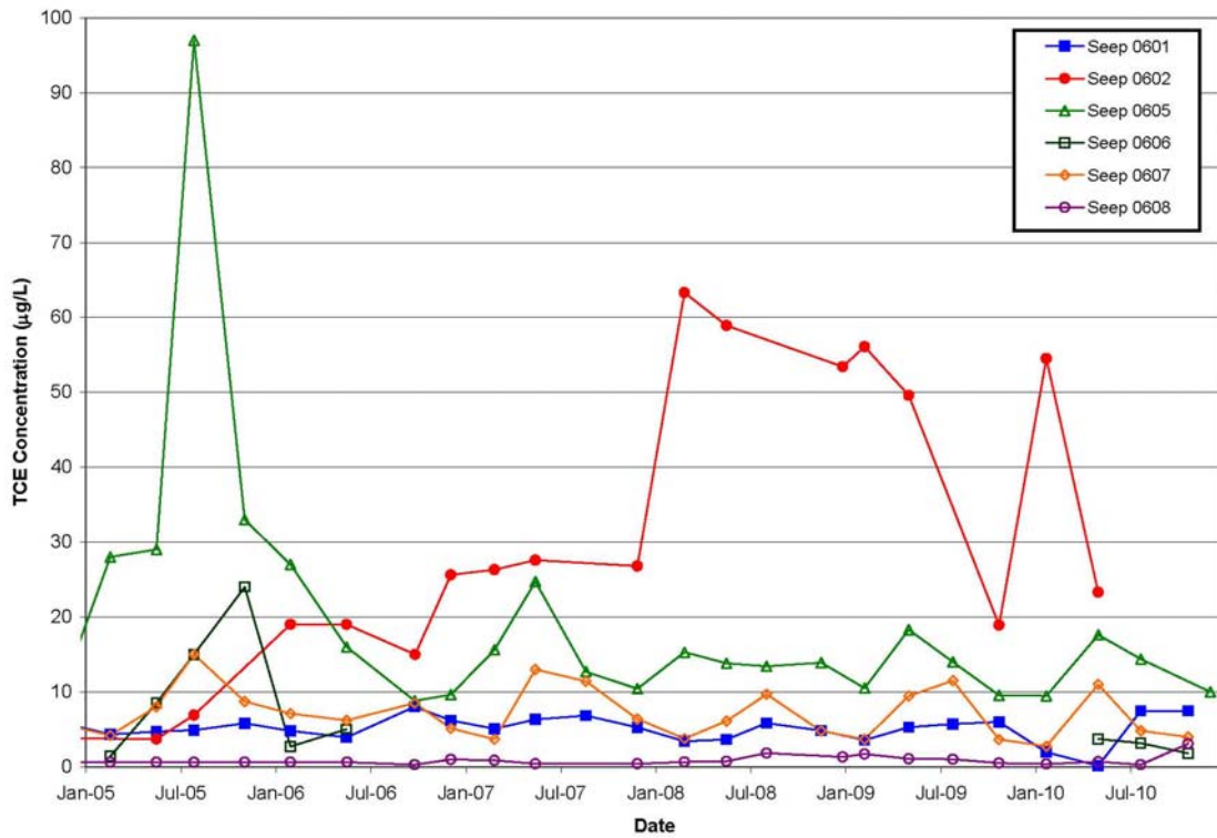
Figure 5. TCE Concentrations in the Main Hill Seeps (2005–2010)
