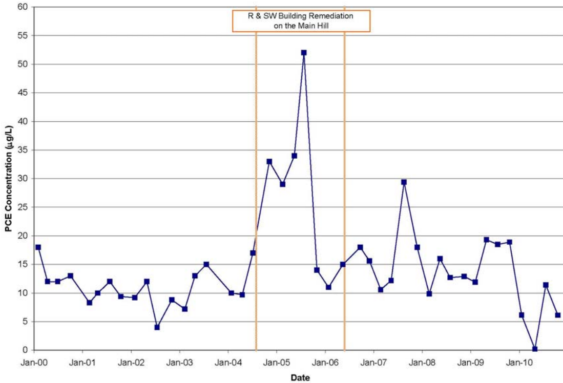
Figure 6. PCE Concentrations in Seep 0601 (2000–2010)
