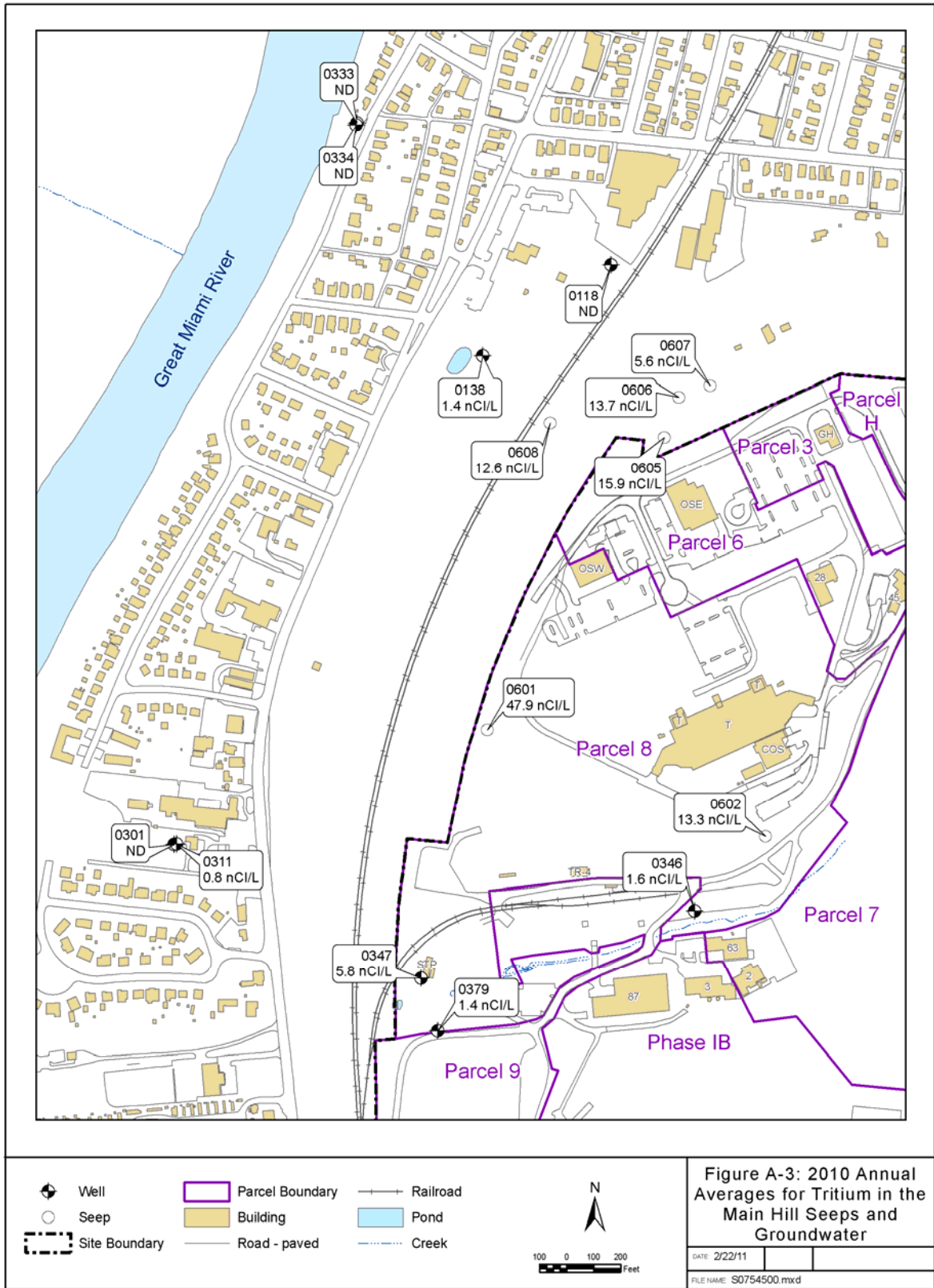
Figure 11. 2010 Annual Average Tritium Levels in the Main Hill Seeps
